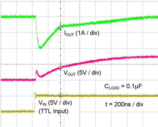
Figure 35. Quasi-Static Source Current with V_{DD} = 8 V
