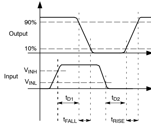
Figure 4. Inverting
