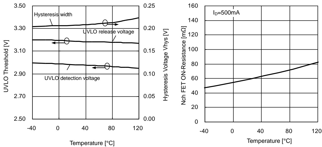
Figure 11. ON-Resistance vs Temperature
