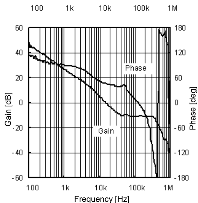
Figure 30. Frequency Response Property 4 ( V_{CC} = 3.5V , I_O = 500mA )
