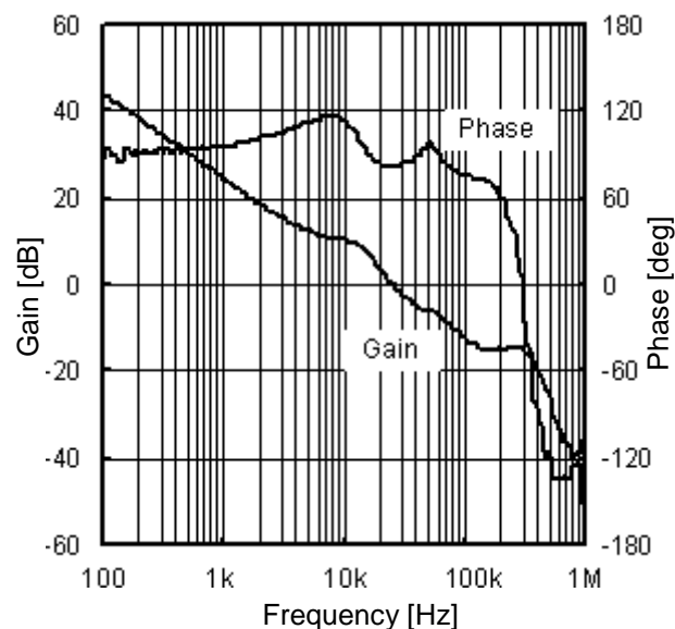
Figure 28. Frequency Response Property 2 ( V_{CC} = 6.0V , I_O = 200mA )
