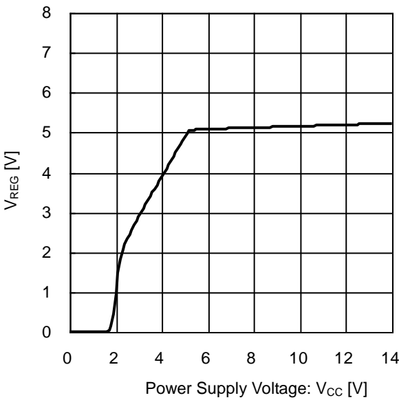
Figure 7. VREG vs Power Supply voltage
