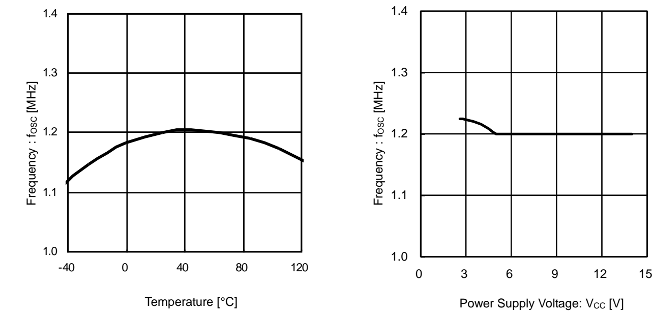
Figure 9. Frequency vs V_{CC}
