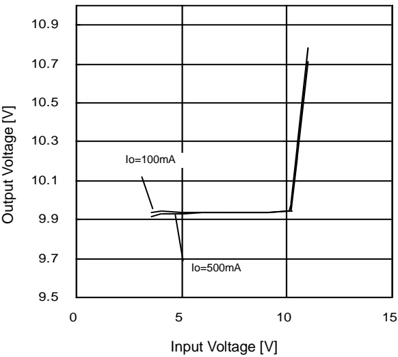
Figure 24. Line Regulation
