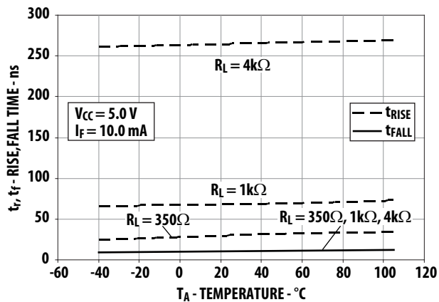
Figure 10. Typical rise and fall time vs. temperature.
