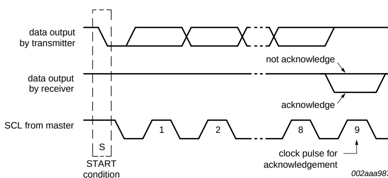
Fig 17. Acknowledgement on the I 2 C-bus
