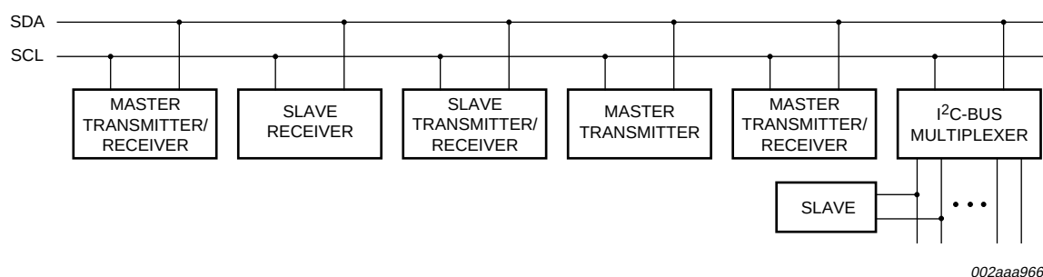
Fig 16. System configuration
