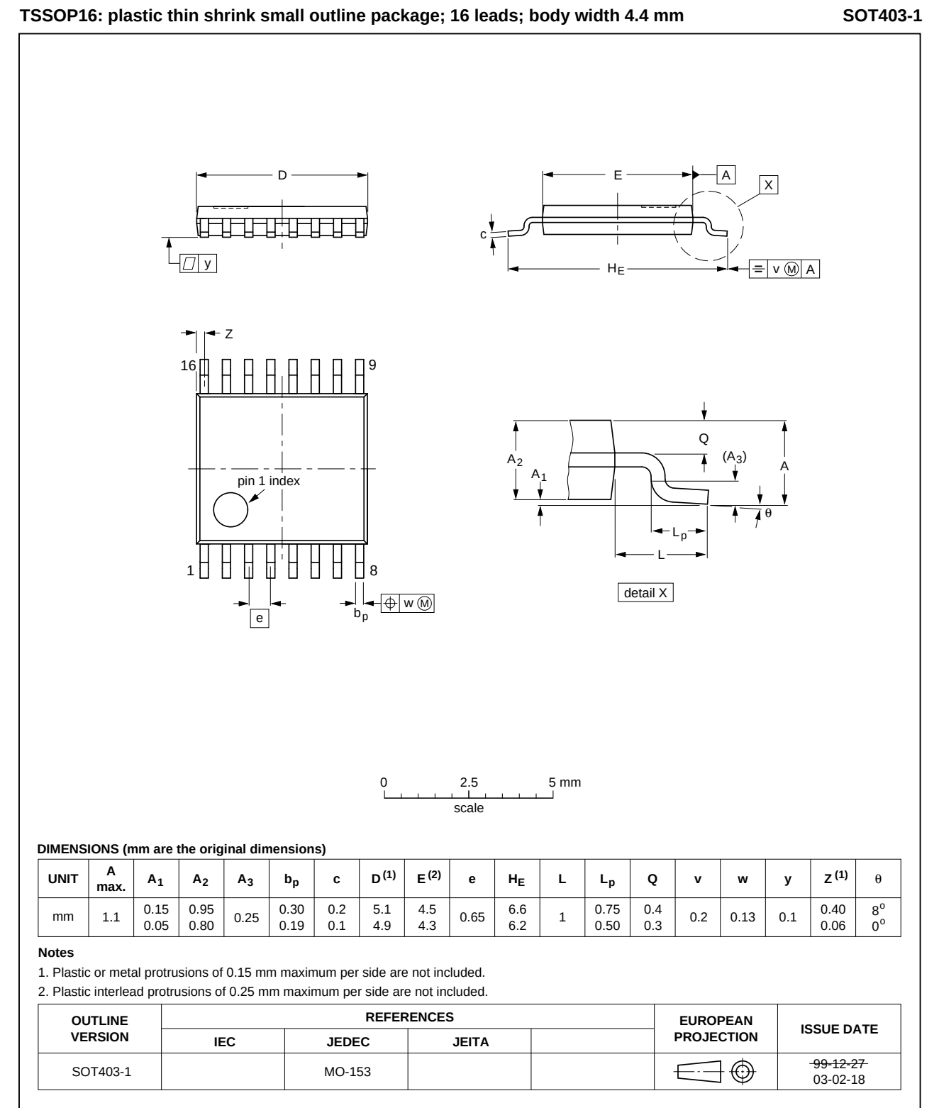
Fig 26. Package outline SOT403-1 (TSSOP16)
