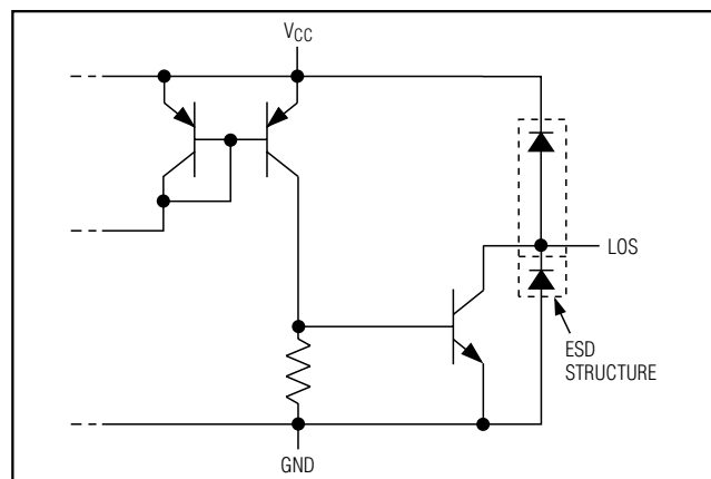
Figure 6. MAX3748A LOS Output Circuit
