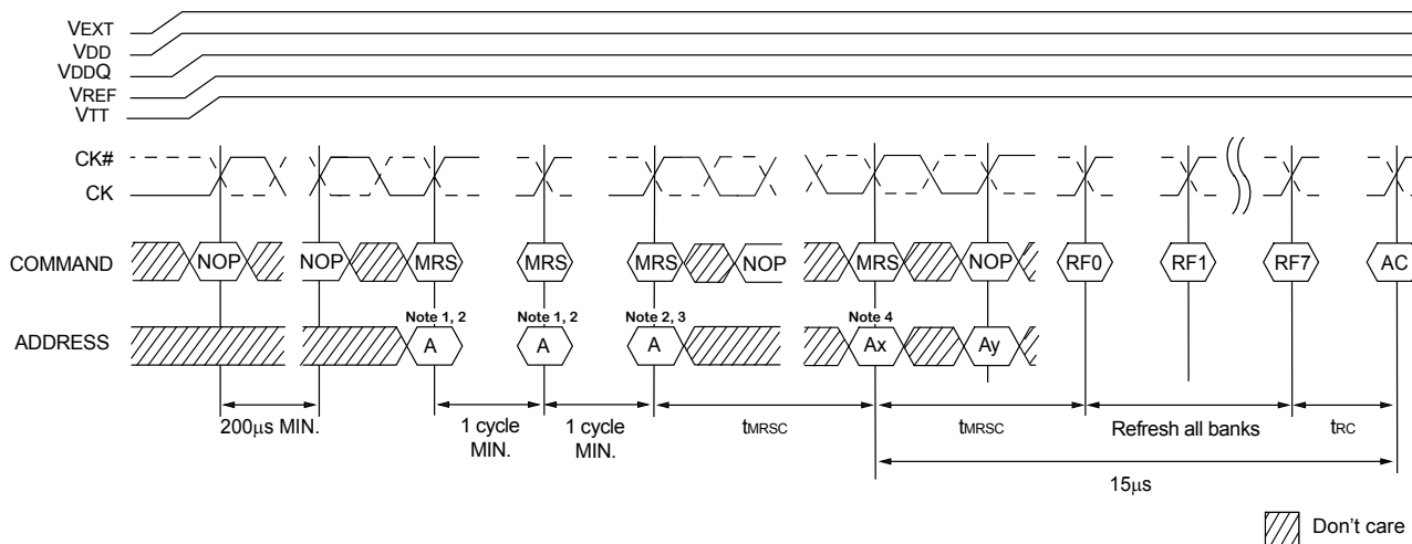
Figure 2-28. Power-Up Sequence in Muxplexed Address Mode
