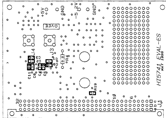
FIGURE 19A. SILKSCREEN
