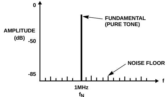
FIGURE 8. FREQUENCY PLOT OF 1MHz TONE
