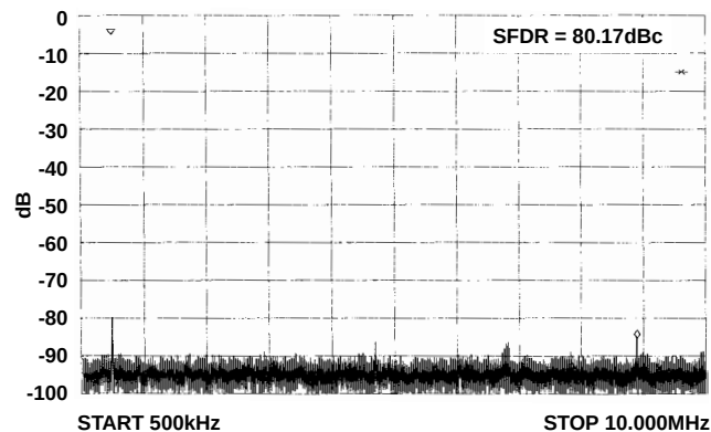
FIGURE 10B. SAMPLE PLOT
