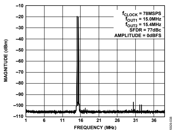
Figure 25. Dual-Tone SFDR
