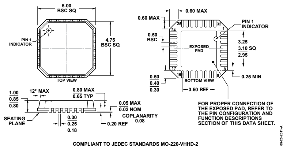
Figure 91. 32-Lead Lead Frame Chip Scale Package [LFCSP_VQ] 5 mm x 5 mm, Very Thin Quad (CP-32-2) Dimensions shown in millimeters
