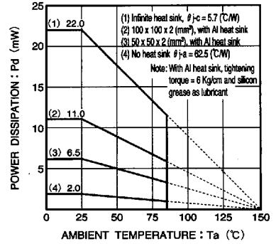
Fig. 3 T_a - power consumption characteristic (TO220)
