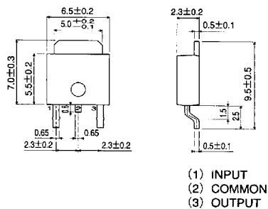
TO252 - 3
