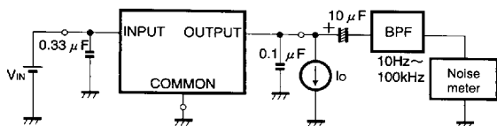
Fig. 7 Measurement circuit for output noise voltage
