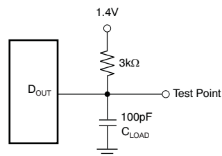
Load Circuit for t_{\text{dto}} , t_{\text{r}} , and t_{\text{f}}
