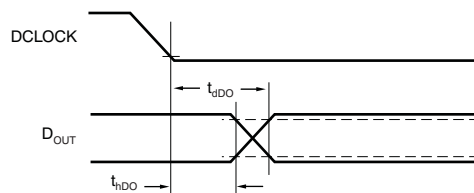
Voltage Waveforms for \text{D}_{\text{OUT}} Delay Times, t_{\text{dto}}
