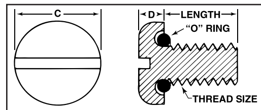
TYPE SL OVERSIZED SLOTTED
