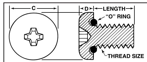
TYPE RM PHILLIPS RECESSED
