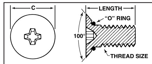
TYPE SFR PHILLIPS RECESSED
