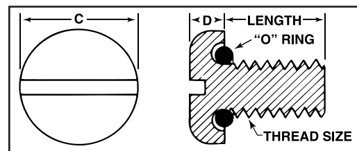
TYPE SM METRIC SLOTTED
