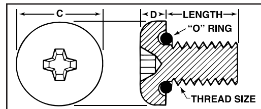
TYPE R PHILLIPS RECESSED (MEETS REQUIREMENTS OF MS 3212 & MS 3213)
