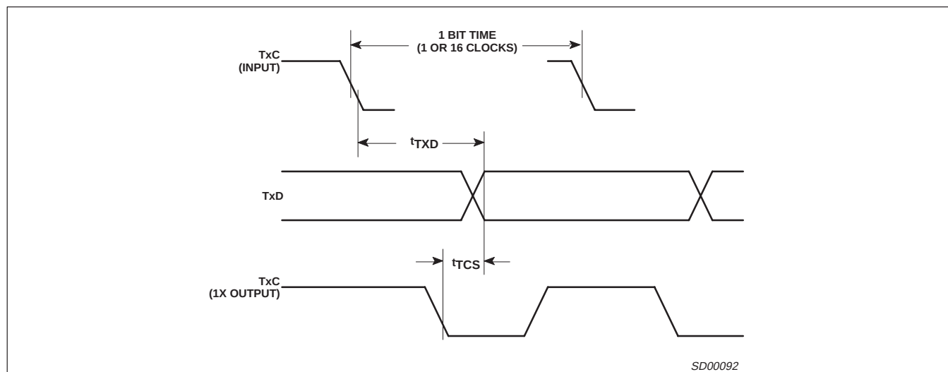
Figure 8. Transmit
