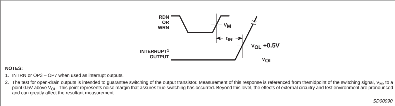
Figure 6. Interrupt Timing
