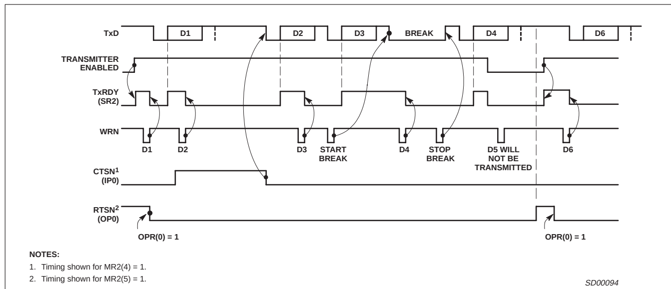
Figure 10. Transmitter Timing
