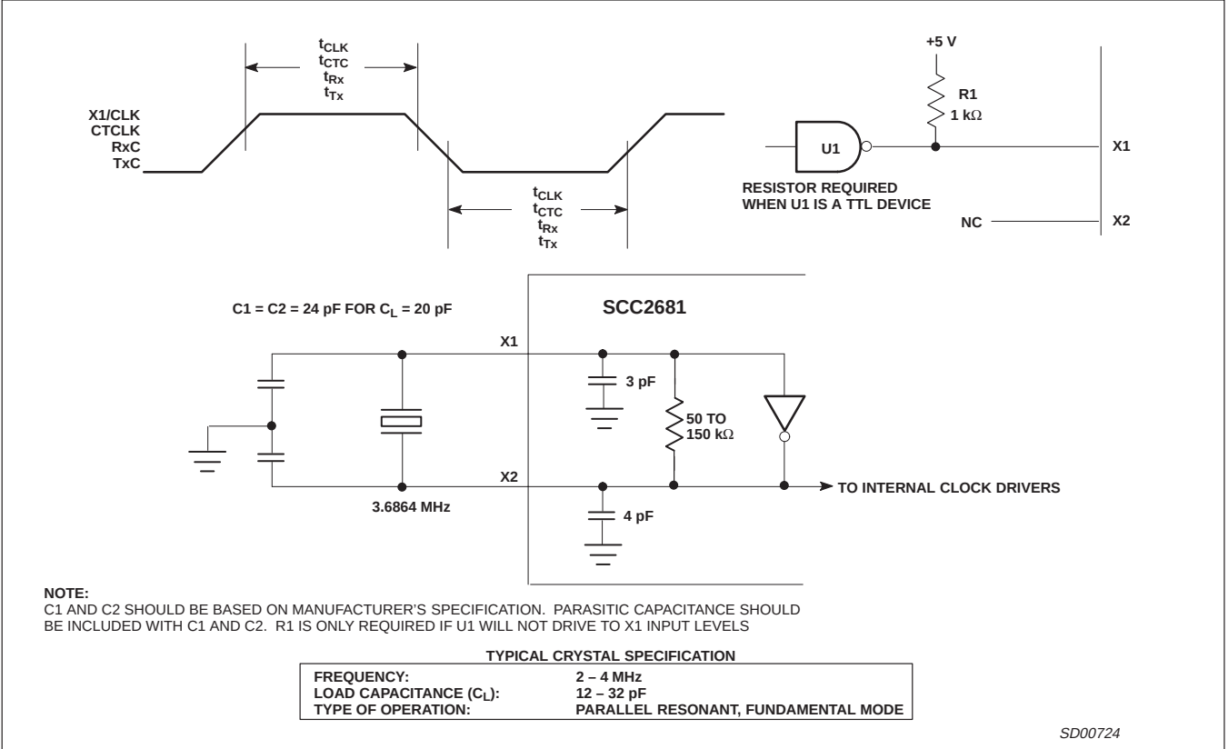
Figure 7. Clock Timing
