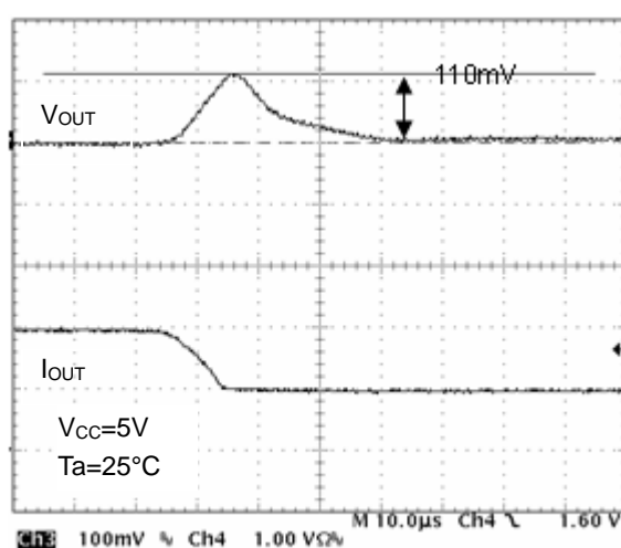
Figure 18. Transient Response (I o =2A to 1A, 10µs)
