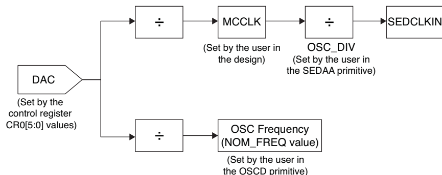
Figure 17-5. Internal Clocking Scheme
