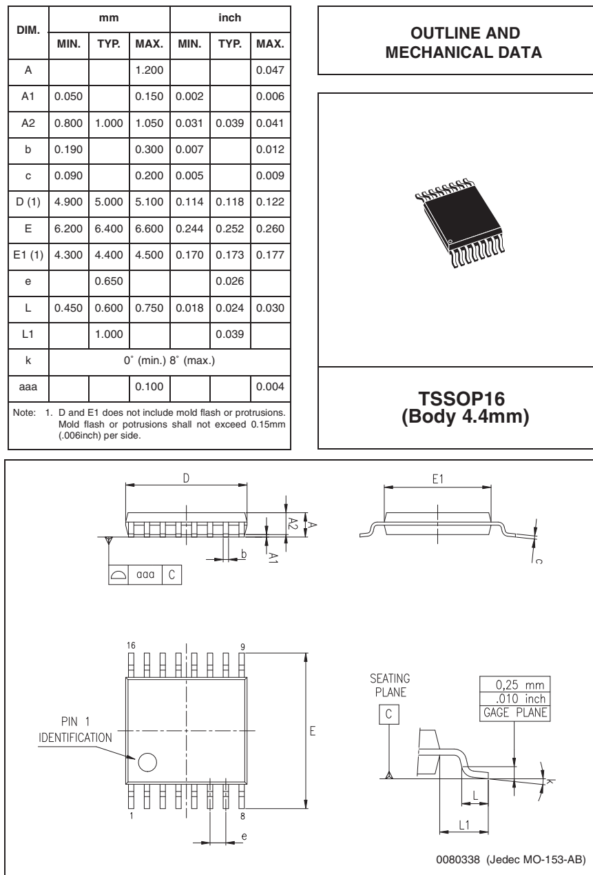
Figure 5. TSSOP16 mechanical data and package dimensions
