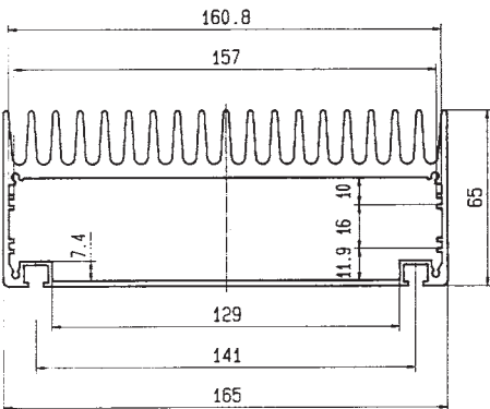
Enclosure Profile
