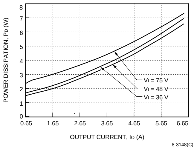
Figure 28. CW030F Power Dissipation vs. Output Current
