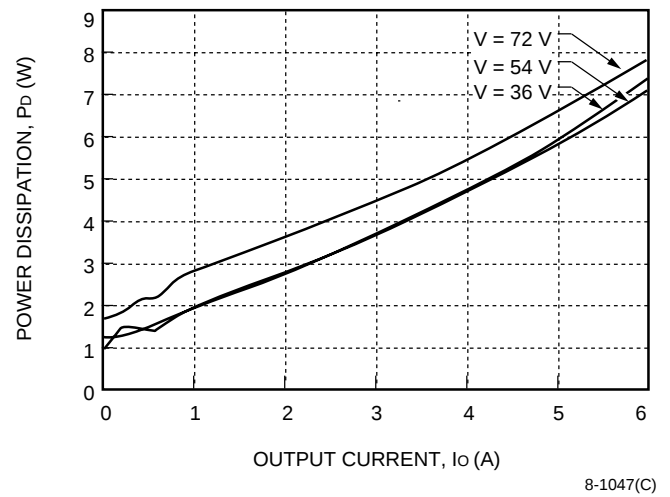
Figure 29. CW030A Power Dissipation vs. Output Current
