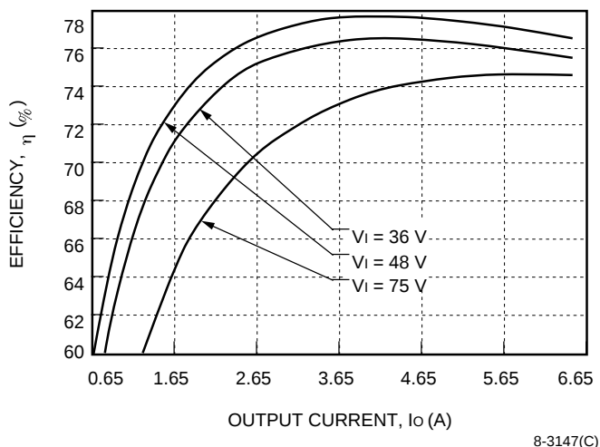
Figure 12. CW030F-M Typical Converter Efficiency vs. Output Current
