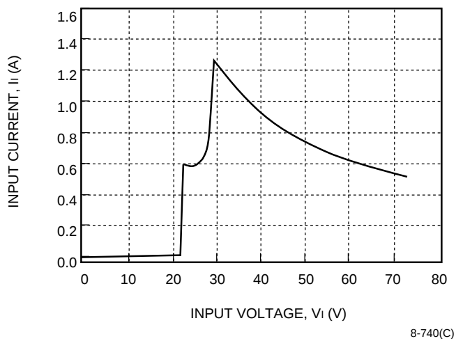
Figure 1. CW030A, B, C Typical Input Characteristics
