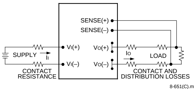
Figure 23. Effective Circuit Configuration for Single-Module Remote-Sense Operation
