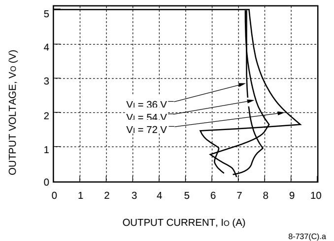
Figure 8. CW030A-M Typical Output Characteristics
