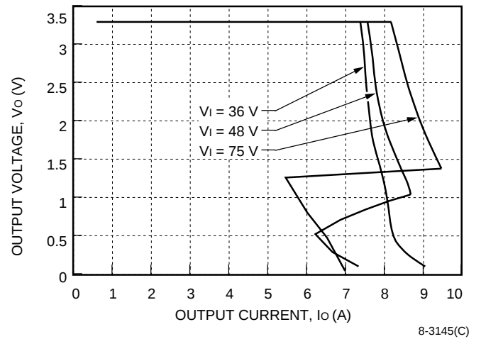
Figure 7. CW030F-M Typical Output Characteristics
