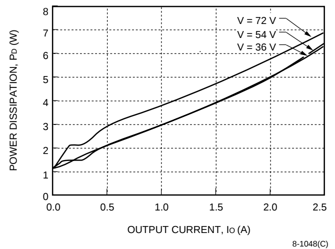
Figure 30. CW030B Power Dissipation vs. Output Current
