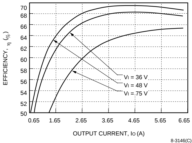
Figure 11. CW030D-M Typical Converter Efficiency vs. Output Current
