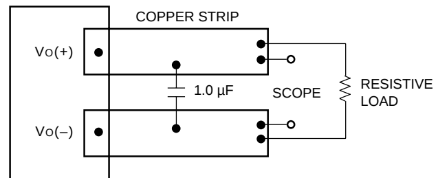
Figure 19. Input Reflected-Ripple Test Setup
