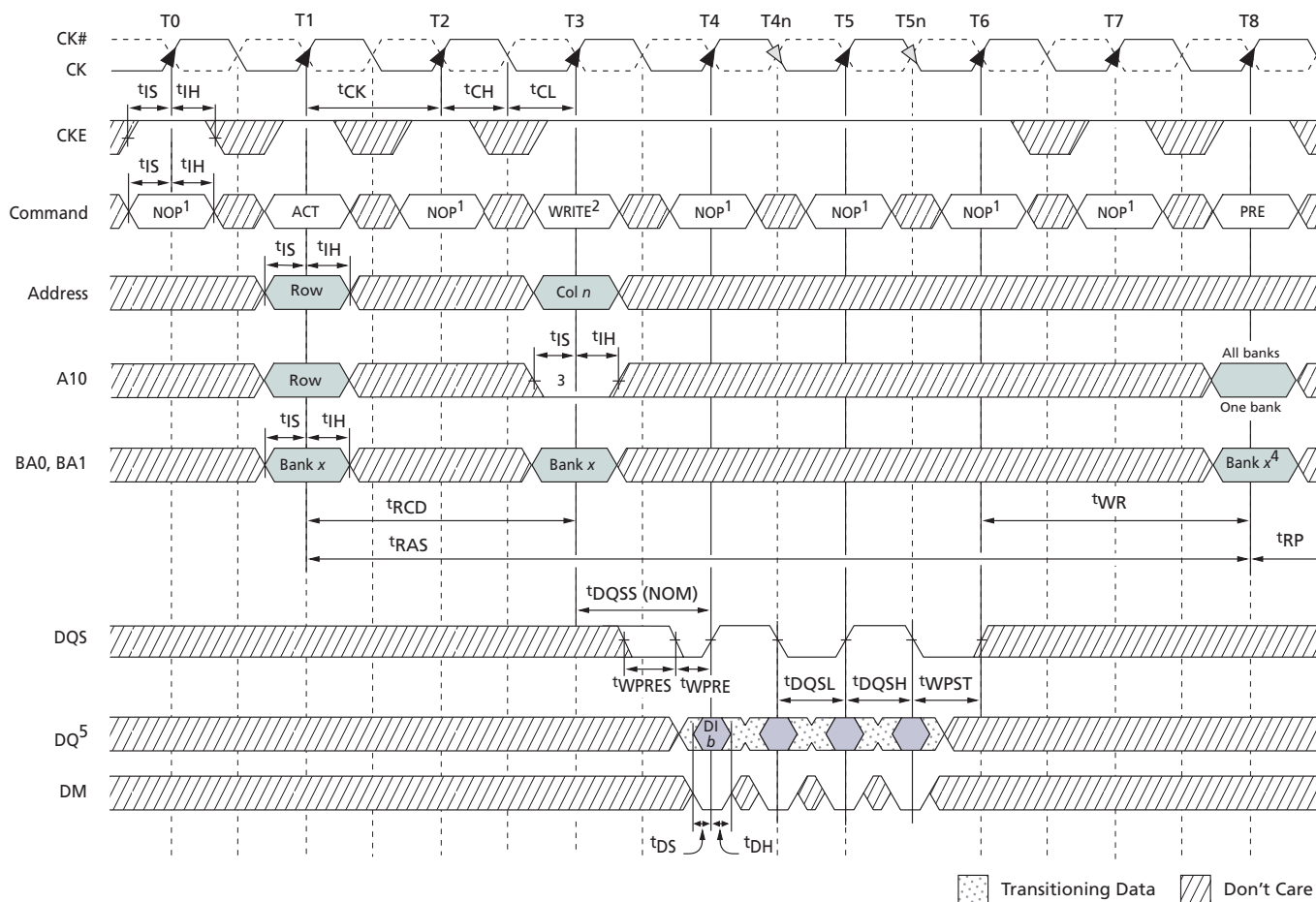
Figure 39: Bank WRITE – Without Auto Precharge
