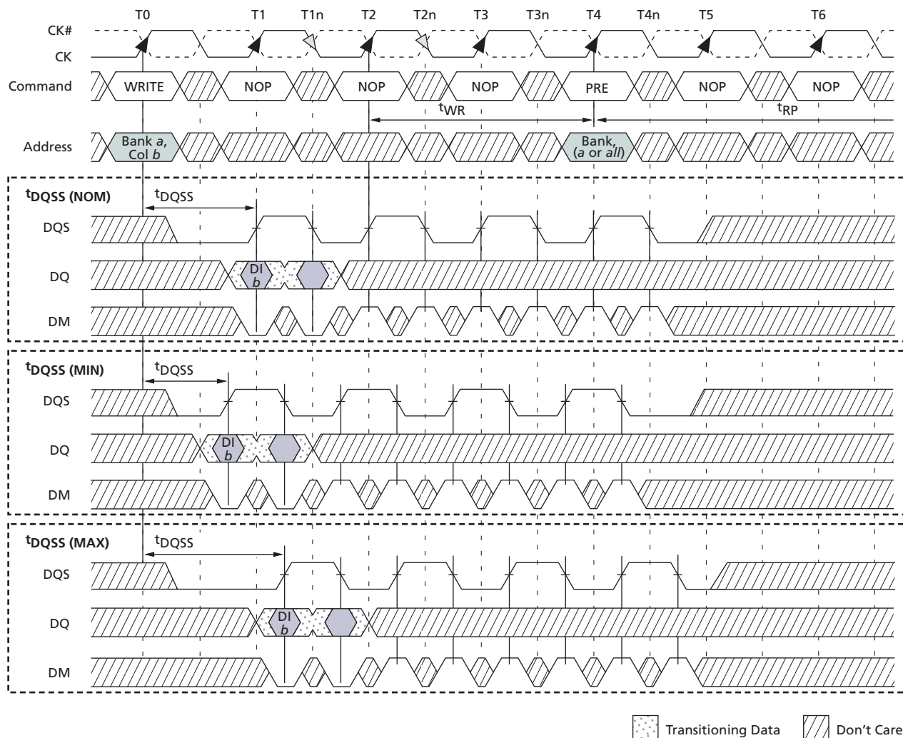
Figure 37: WRITE-to-PRECHARGE – Interrupting
