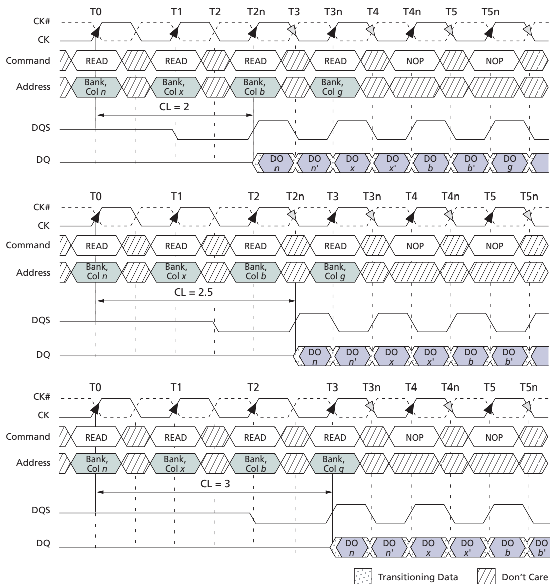
Figure 21: Random READ Accesses
