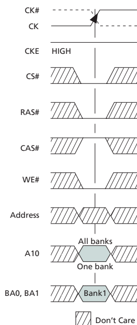
Figure 11: PRECHARGE Command
