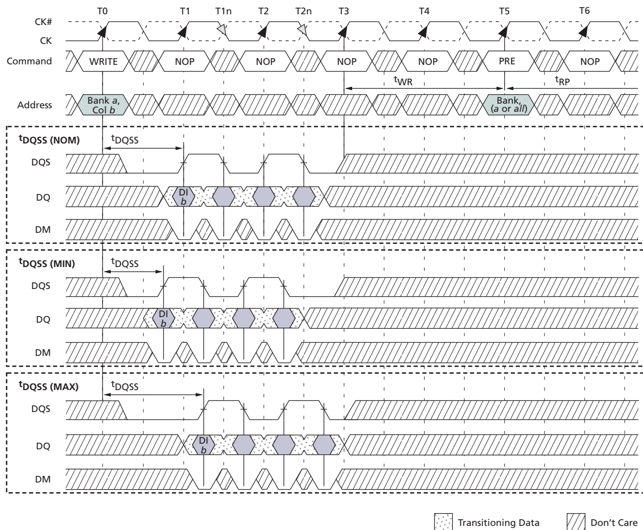
Figure 36: WRITE-to-PRECHARGE – Uninterrupting
