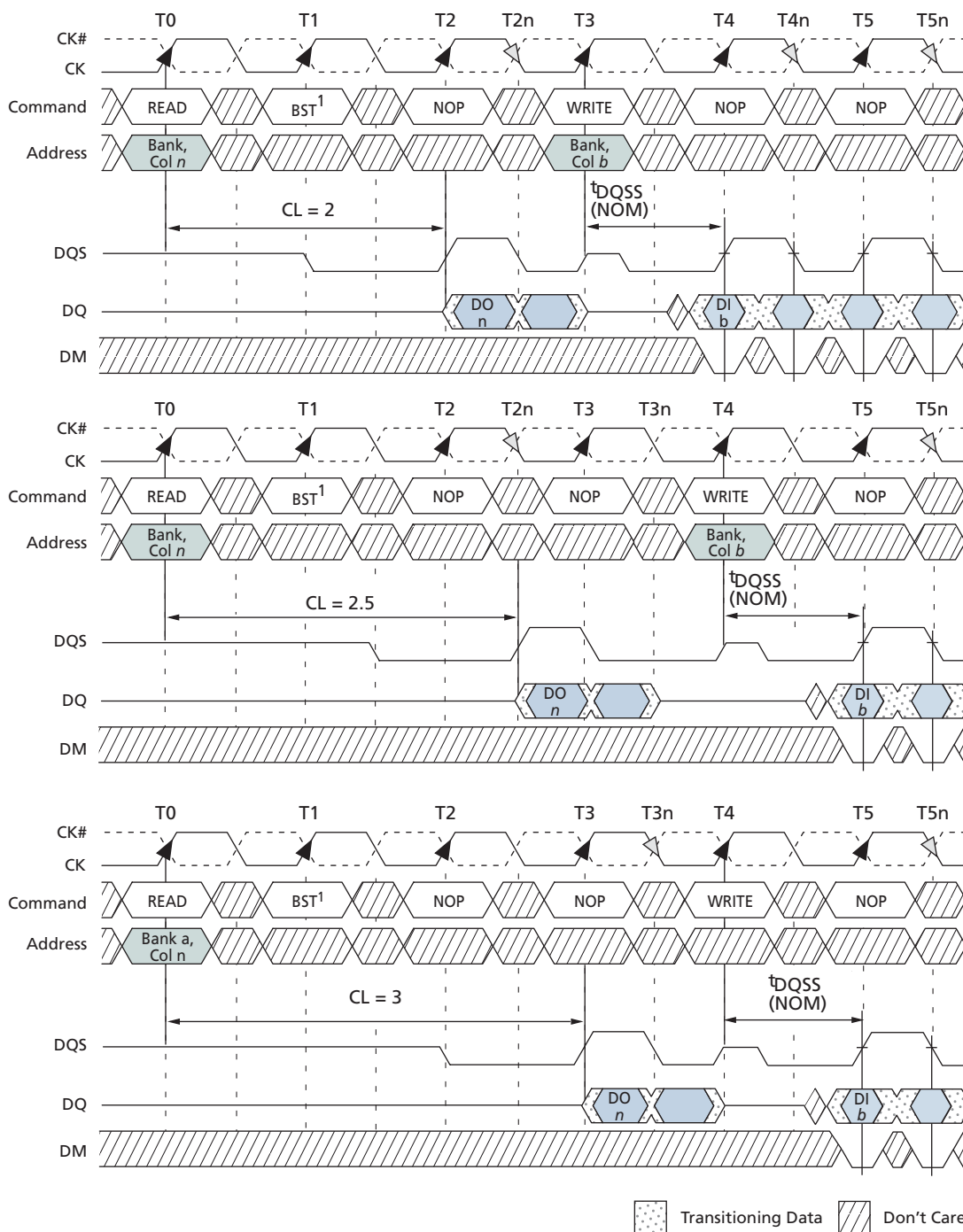
Figure 23: READ-to-WRITE
