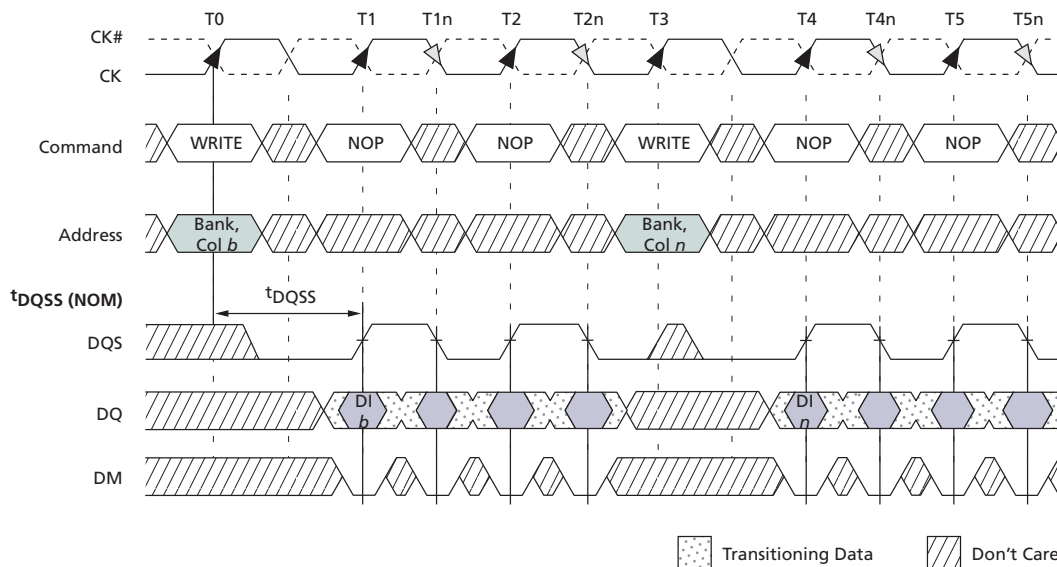
Figure 31: Nonconsecutive WRITE-to-WRITE
