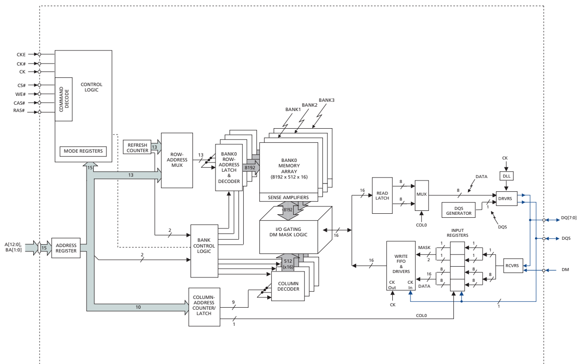
Figure 3: 16 Meg x 16 Functional Block Diagram
