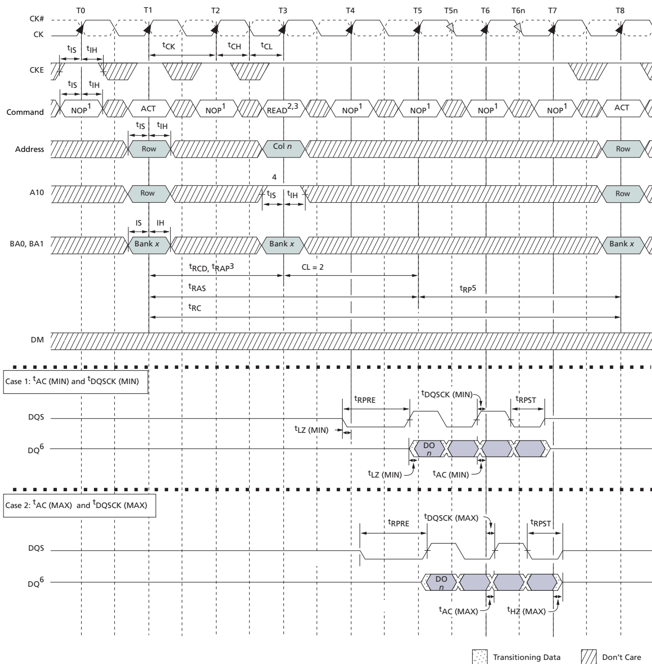
Figure 42: Bank READ – with Auto Precharge
