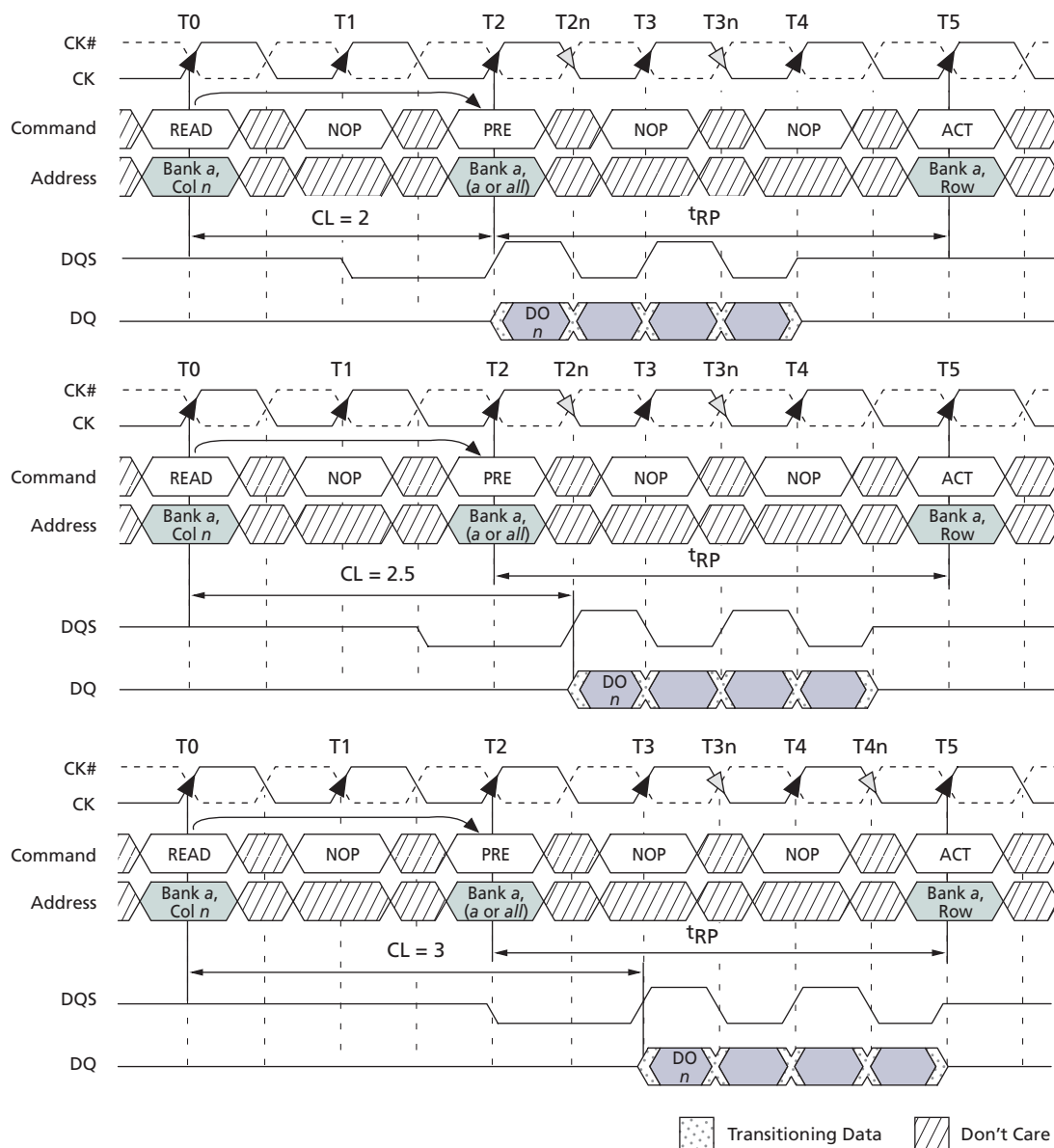
Figure 24: READ-to-PRECHARGE
