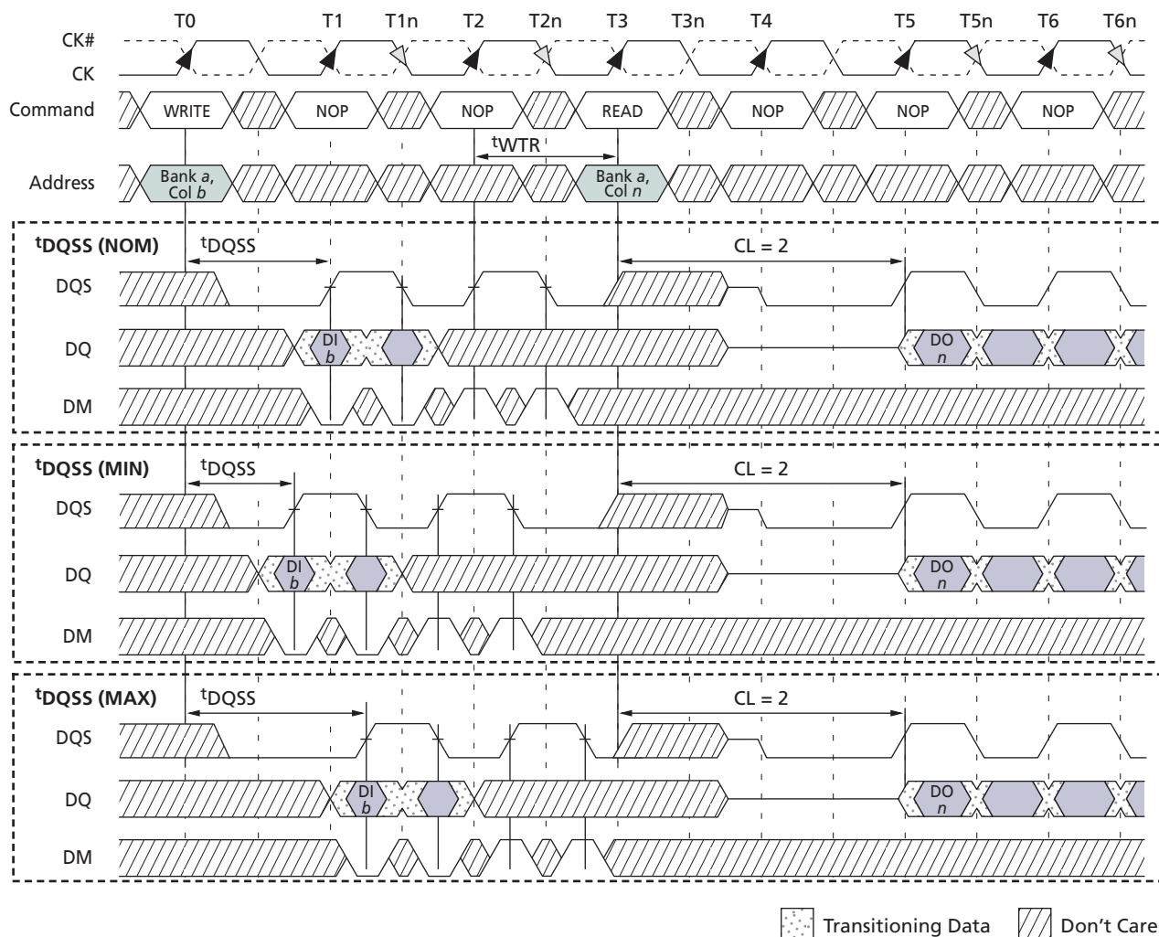
Figure 34: WRITE-to-READ – Interrupting
