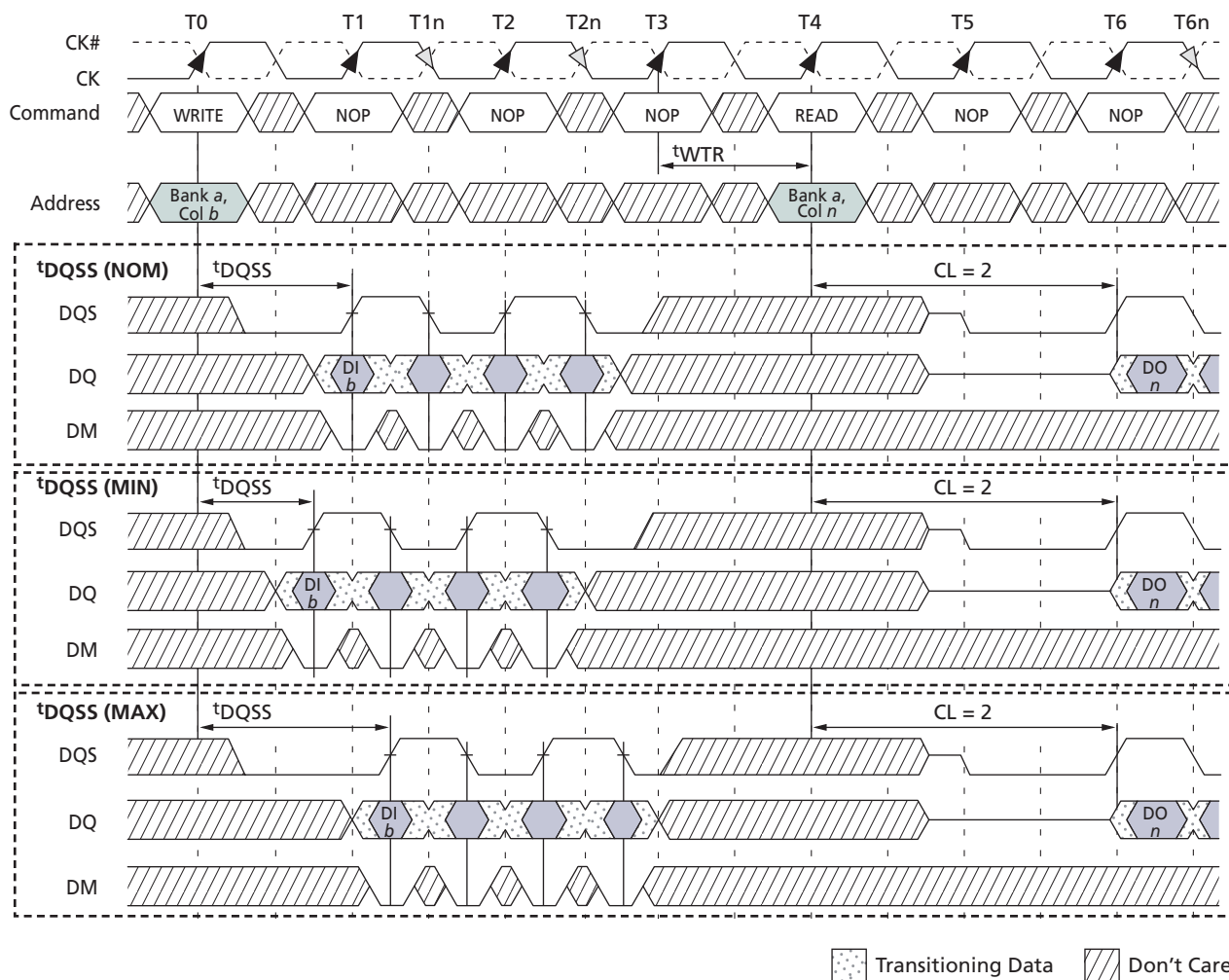
Figure 33: WRITE-to-READ – Uninterrupting
