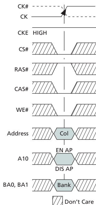
Figure 10: WRITE Command
