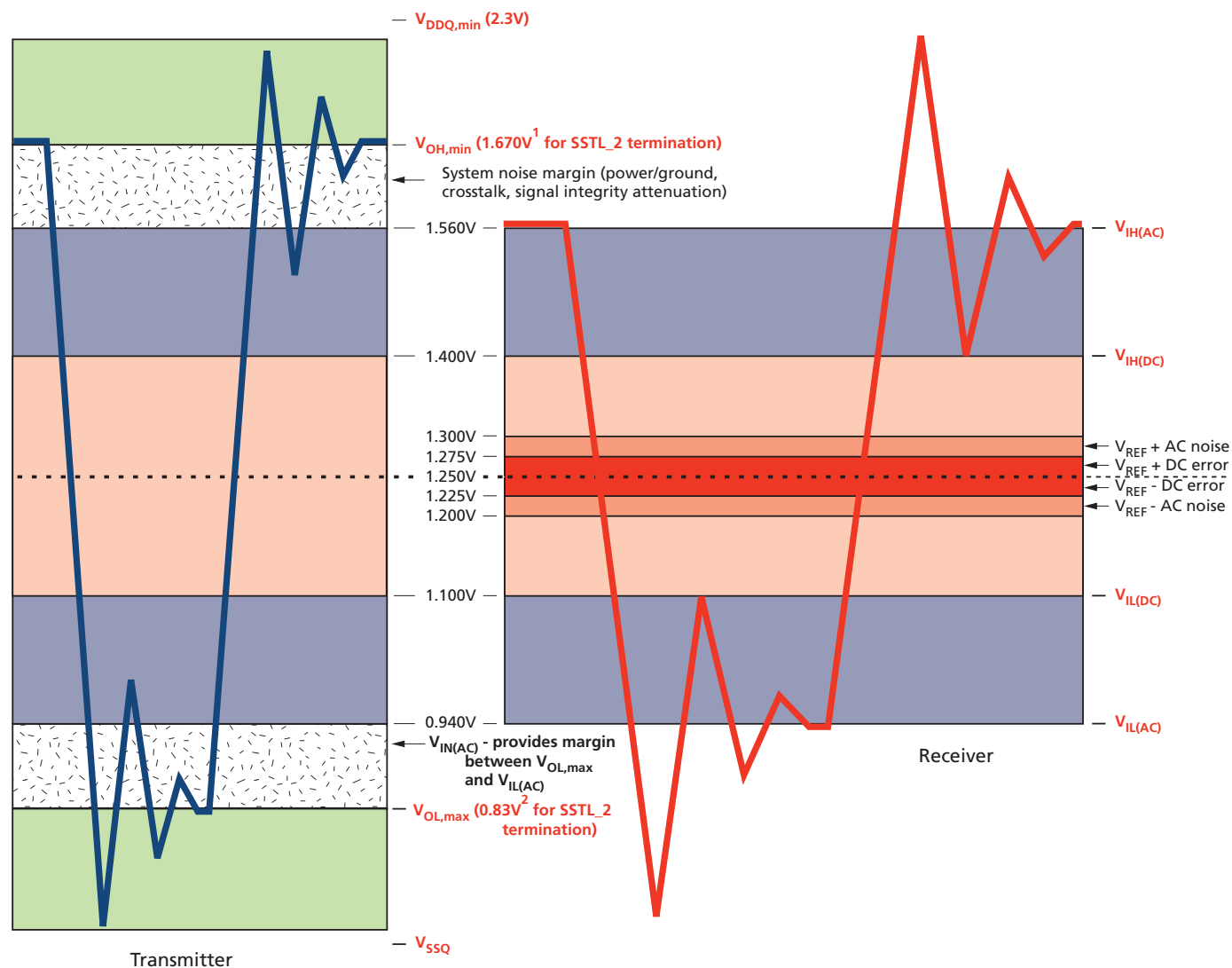
Figure 1: Input Voltage Waveform
