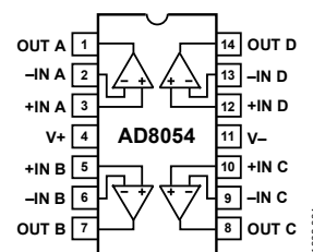
Figure 4. SOIC (R-14) and TSSOP (RU-14)
