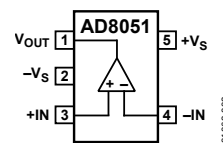
Figure 2. SOT-23-5 (RJ)
