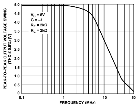
Figure 5. Low Distortion Rail-to-Rail Output Swing
