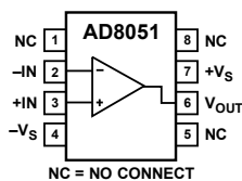
Figure 1. SOIC-8 (R)
