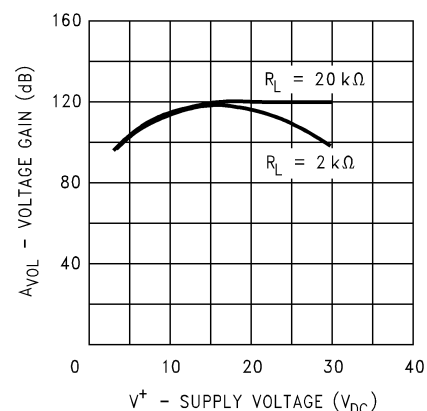
Voltage Gain
