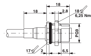
Dimensioned drawing
