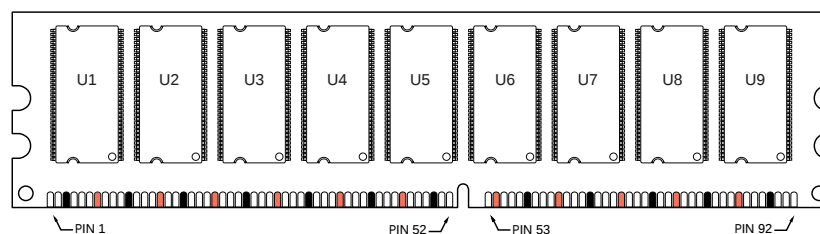
Figure 2: Pin Locations: 184-PIN DIMM
