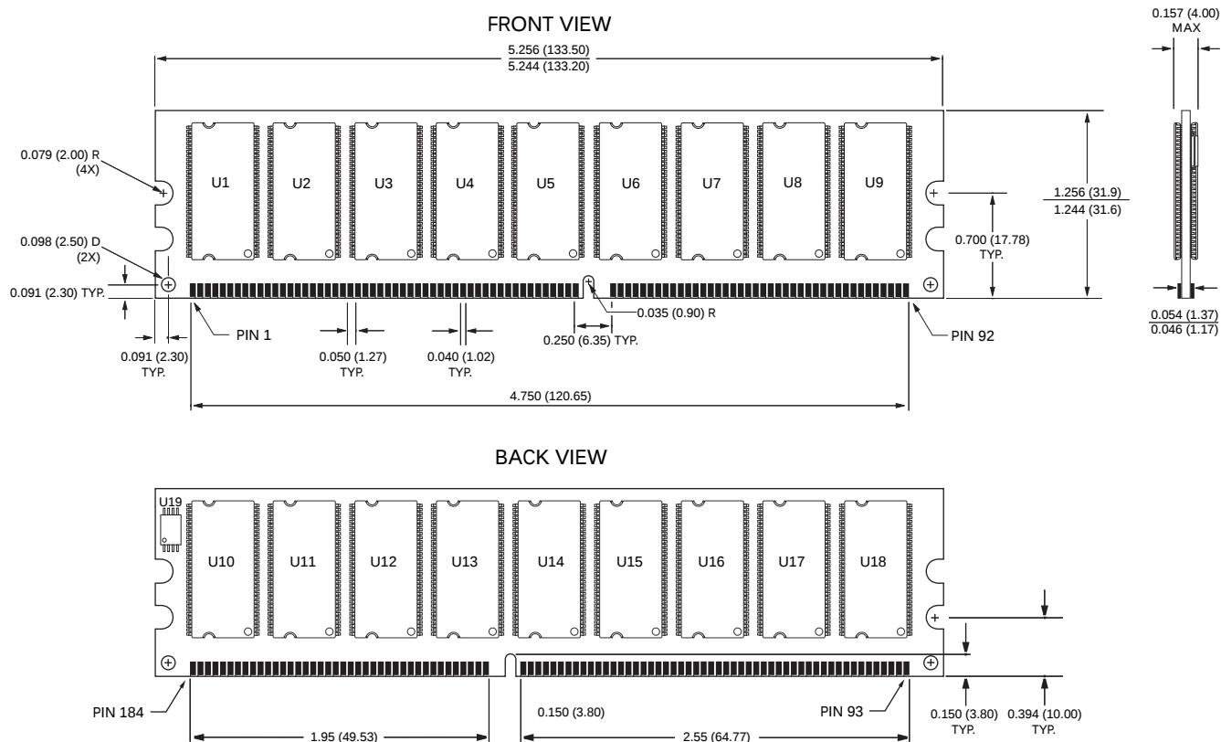
Figure 15: 184-PIN DIMM Dimensions
