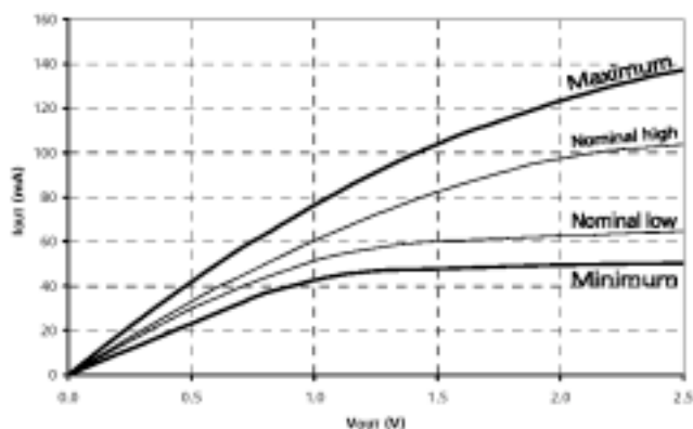
Figure 7: Pull-Down Characteristics
