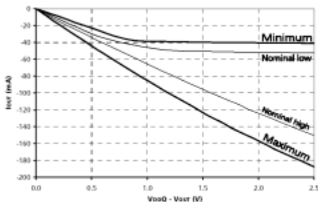
Figure 8: Pull-Up Characteristics
