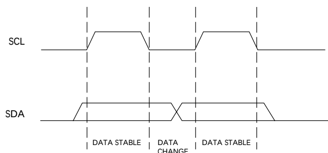
Figure 11: Data Validity
