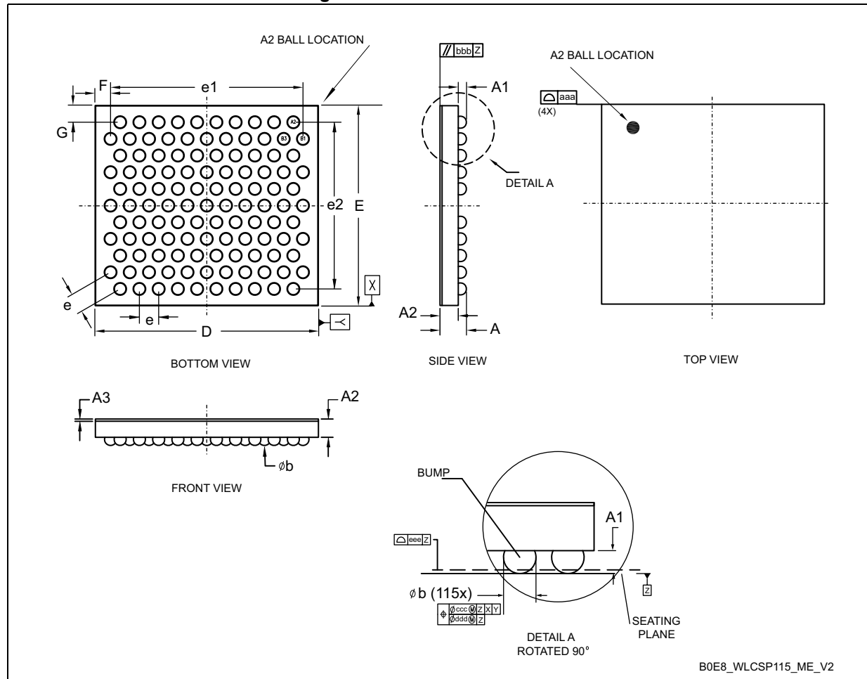
Figure 70. WLCSP115 - Outline
