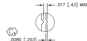
CRIMP DETAIL SCALE: 2x (TYP- ALL CRIMPS)
