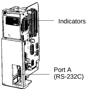
C200HW-COM02
