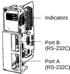
C200HW-COM05-E
