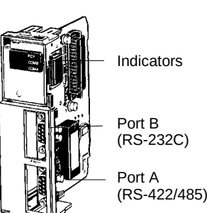
C200HW-COM06-E
