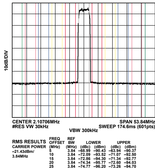
Figure 27. Typical Single-Carrier WCDMA ACLR Performance at 2.1 GHz, f_{DAC} = 2457.6 MSPS (Second Nyquist Zone)
