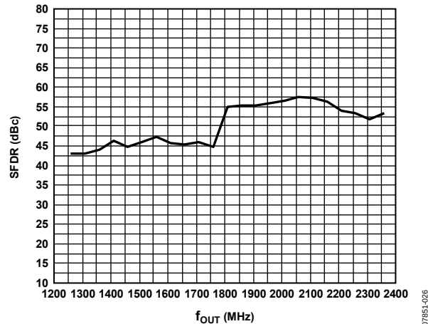
Figure 26. SFDR in Mix Mode vs. f_{OUT} at 2.4 GSPS
