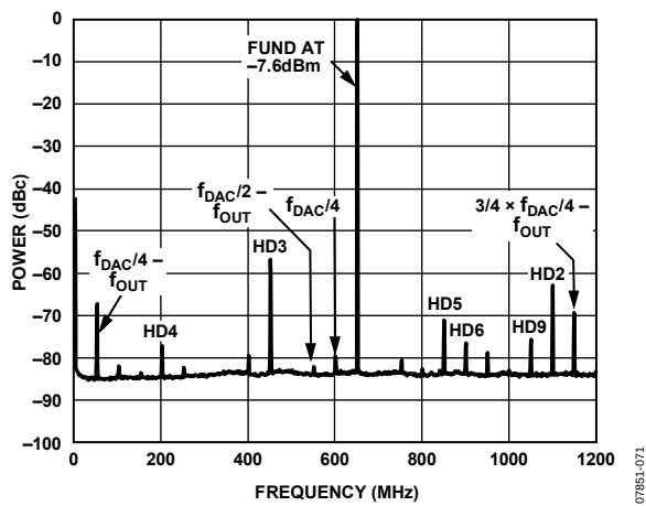
Figure 70. Spectral Plot
