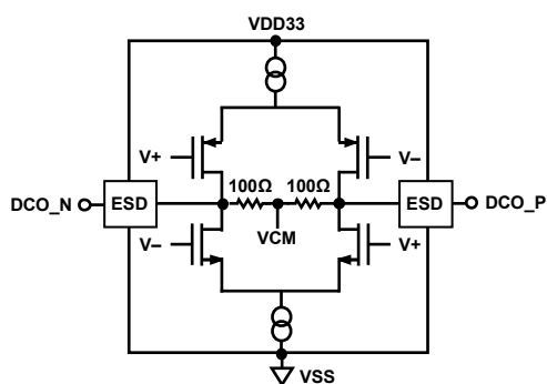
Figure 44. Equivalent LVDS Output
