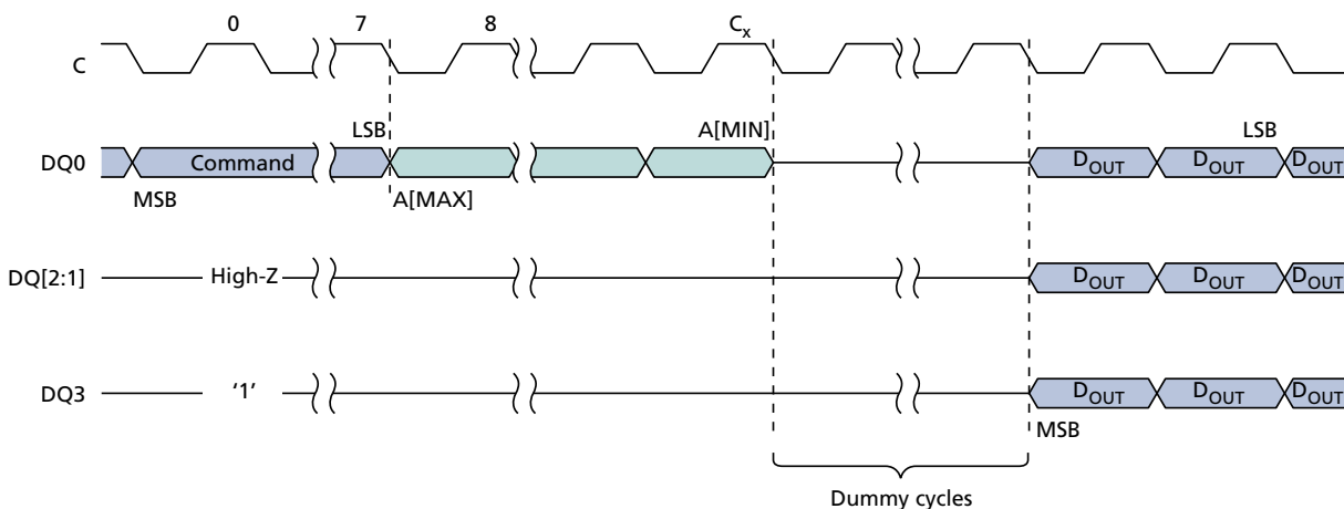
Figure 19: QUAD OUTPUT FAST READ Command – STR
