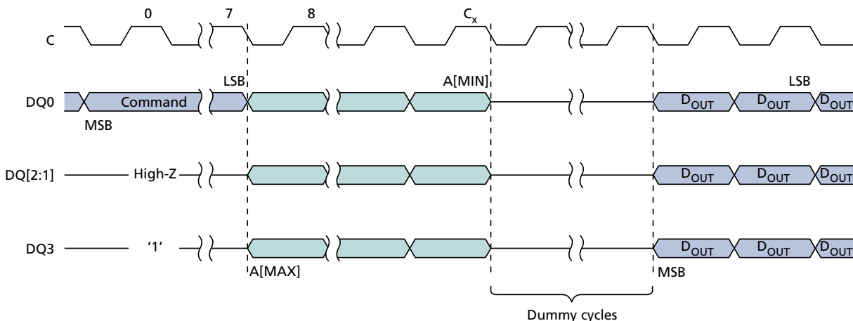
Figure 20: QUAD INPUT/OUTPUT FAST READ Command – STR
