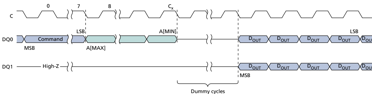
Figure 17: DUAL OUTPUT FAST READ Command – STR
