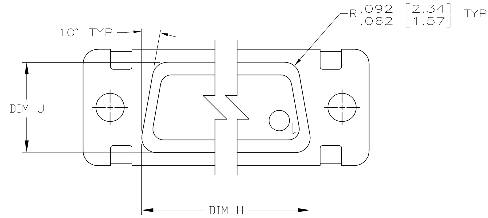
VIEW Z-Z
