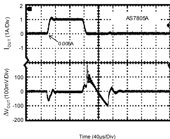
Load Transient (Conditions: V_{IN} = 10\text{V} , C_{IN} = 0.33\mu\text{F} , C_{OUT} = 0.1\mu\text{F} )
