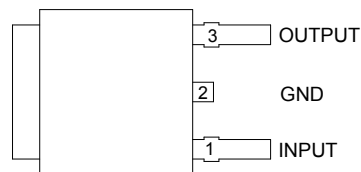
(TO-252-2 (5))
