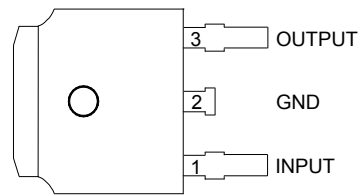
(TO-252-2 (3)) (Option 2)
