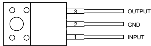
TF Package (TO-220F-3)
