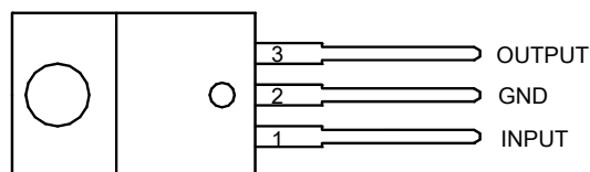
T Package (TO-220-3) (Option 2)
