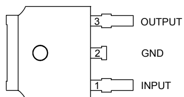
(TO-252-2 (3)) (Option 1)
