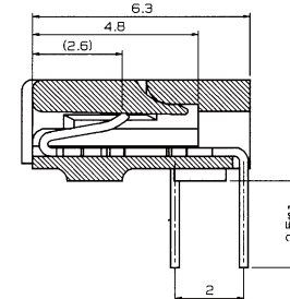
SECT. X-X
