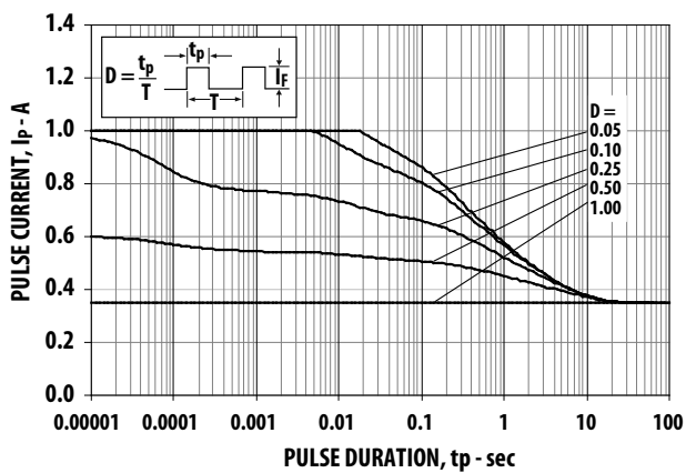
Figure 6. Maximum pulse current vs. pulse duration. Derated based on T_A = 25^\circ\text{C} , R\theta_{JA} = 50^\circ\text{C/W} .
