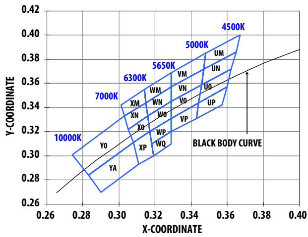
Figure 27. Color bin structure for Cool White.
