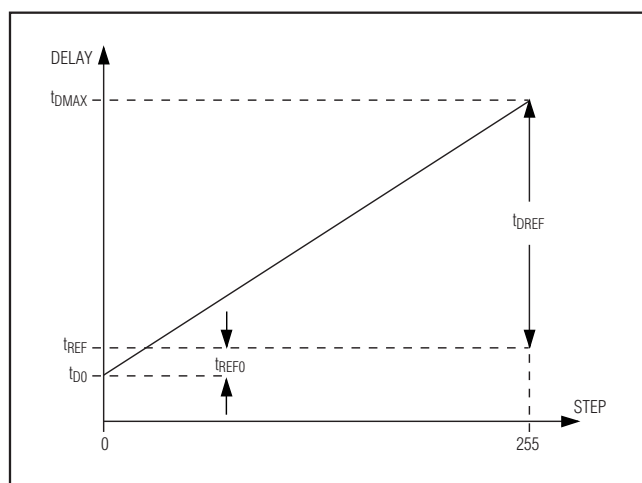
Figure 8. Delay Parameters
