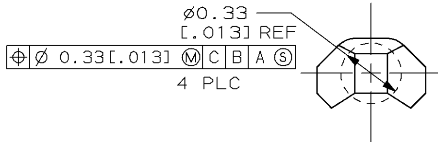
DETAIL C SCALE 50:1
