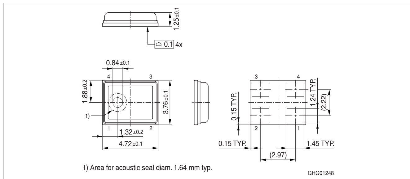
Figure 10 Package outline
