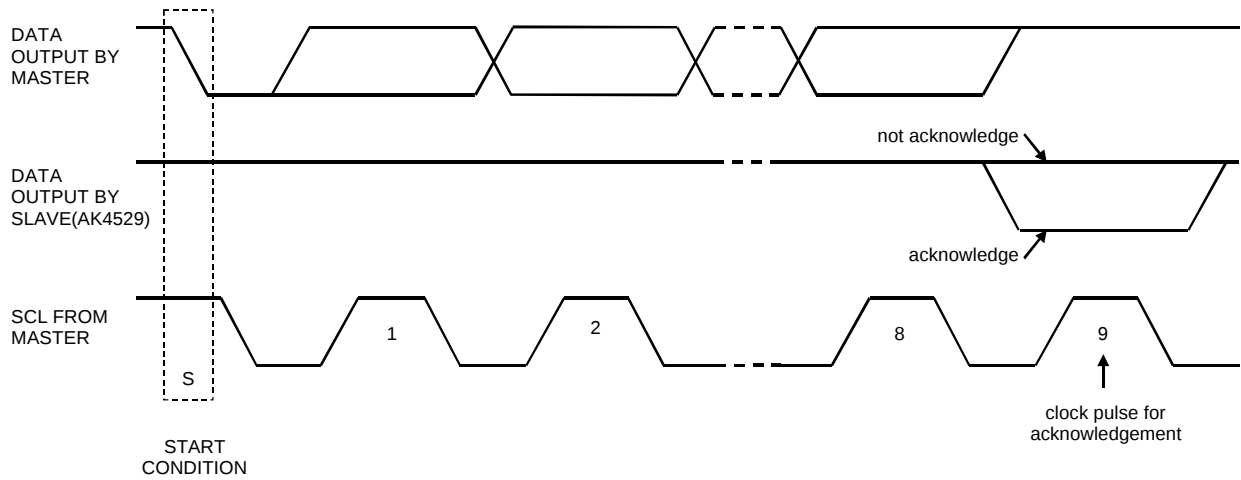
Figure 18. Acknowledge on the I²C-bus
