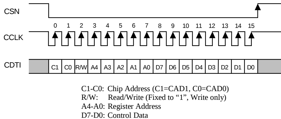
Figure 12. 3-wire Serial Control I/F Timing
