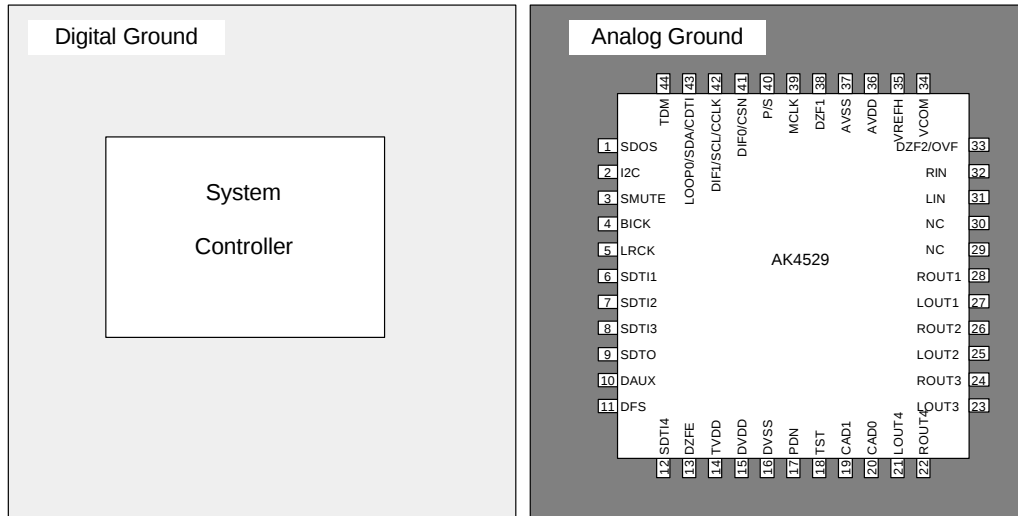
Figure 21. Ground Layout
