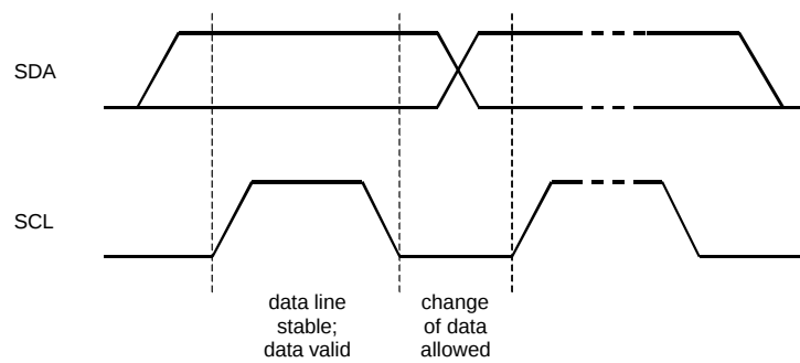
Figure 19. Bit transfer on the I²C-bus
