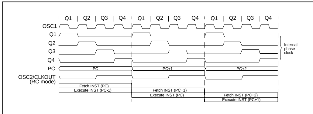
FIGURE 3-2: CLOCK/INSTRUCTION CYCLE
