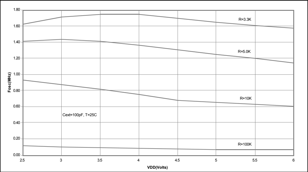
FIGURE 20-3: TYPICAL RC OSCILLATOR FREQUENCY vs. V_{DD} , C_{EXT} = 100\text{ pF}
