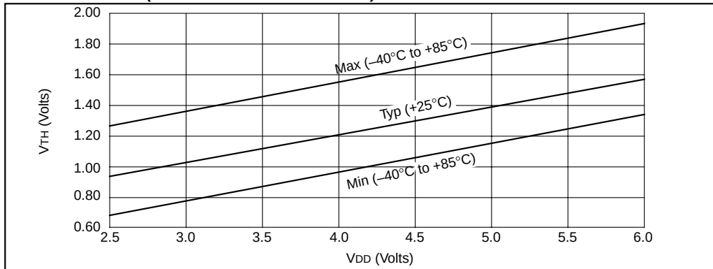
FIGURE 12-10: V_{IH} , V_{IL} OF \overline{MCLR} , T0CKI AND OSC1 (IN RC MODE) vs. V_{DD}
