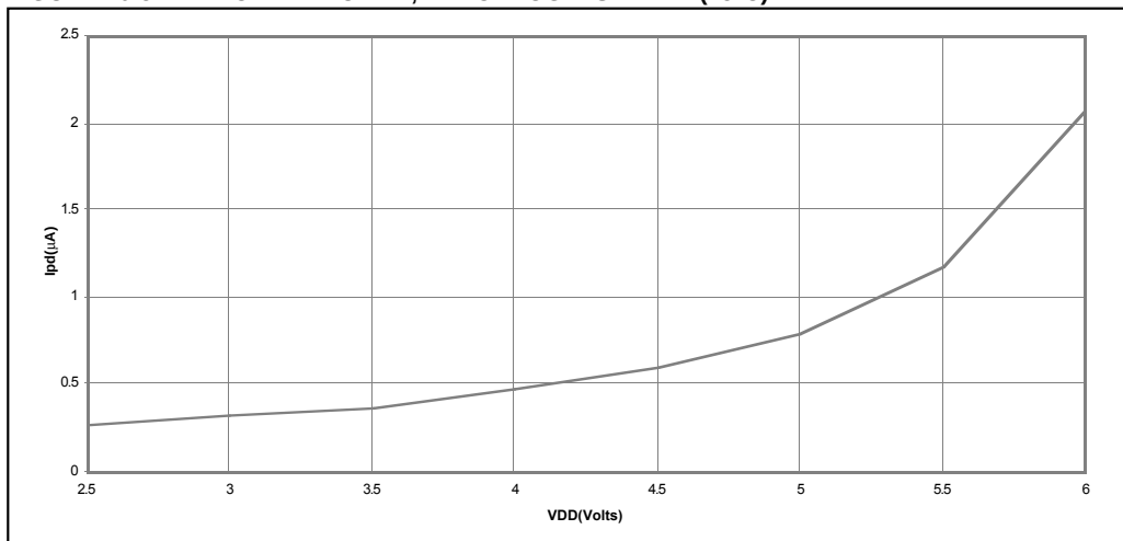
FIGURE 20-5: TYPICAL I_{PD} vs. V_{DD} , WATCHDOG DISABLED ( 25^{\circ}\text{C} )
