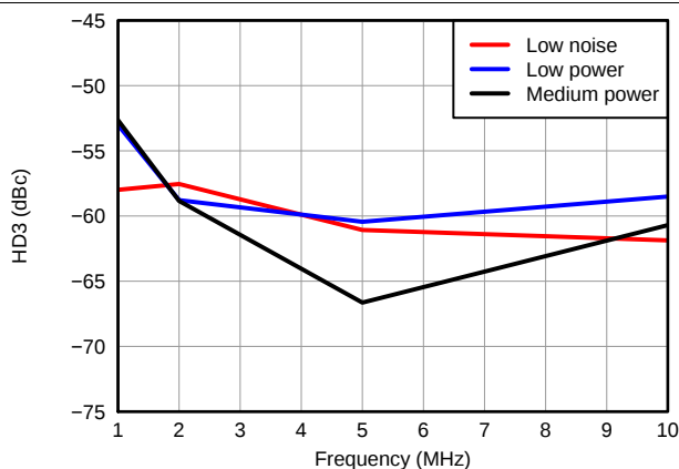
Figure 38. HD3 vs Frequency, V_{\text{IN}} = 500 mVpp and V_{\text{OUT}} = -1 dBFS
