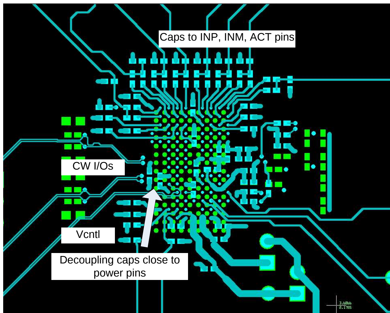
Figure 114. Layout Example
