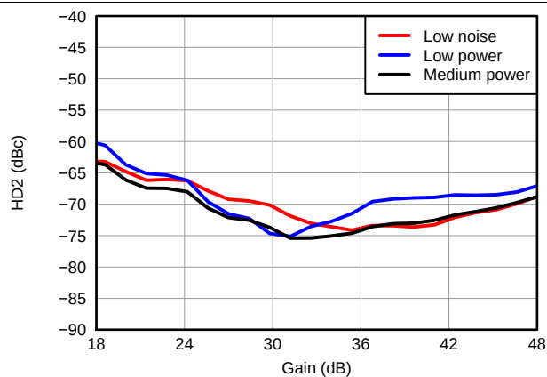
Figure 43. HD2 vs Gain, LNA = 24 dB and PGA = 24 dB and V_{\text{OUT}} = -1 dBFS
