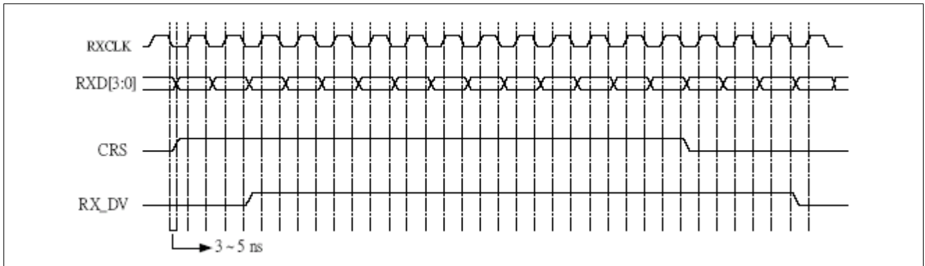
Figure 16 Timing
