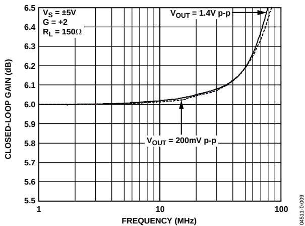
Figure 13. 0.1 dB Flatness (SOIC)
