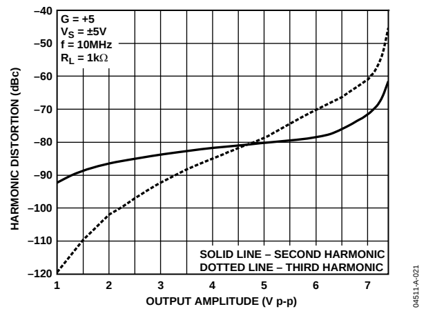
Figure 34. Harmonic Distortion vs. Output Amplitude (CSP)
