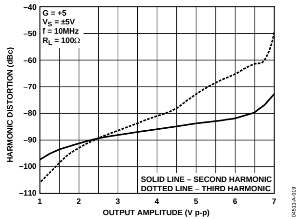
Figure 33. Harmonic Distortion vs. Output Amplitude (CSP)
