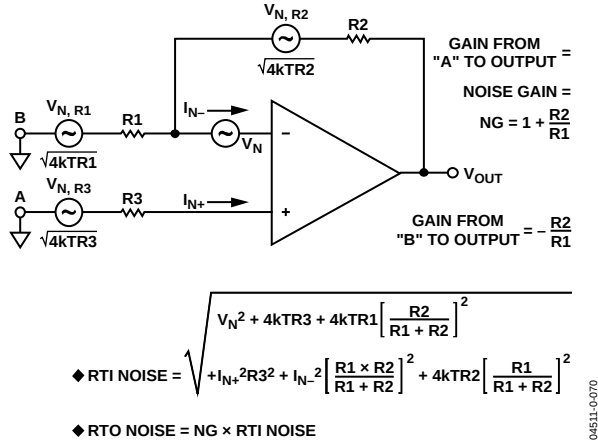
Figure 69. Op Amp Noise Analysis Model
