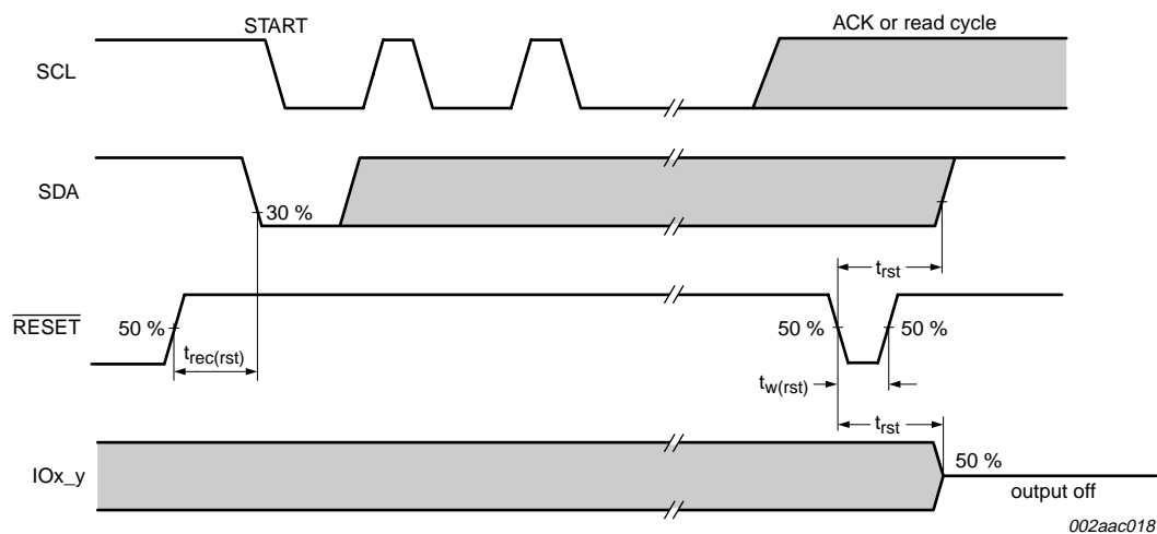
Fig 18. Reset timing
