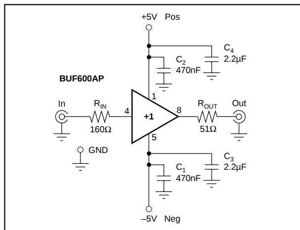
FIGURE 2. Test Circuit.
