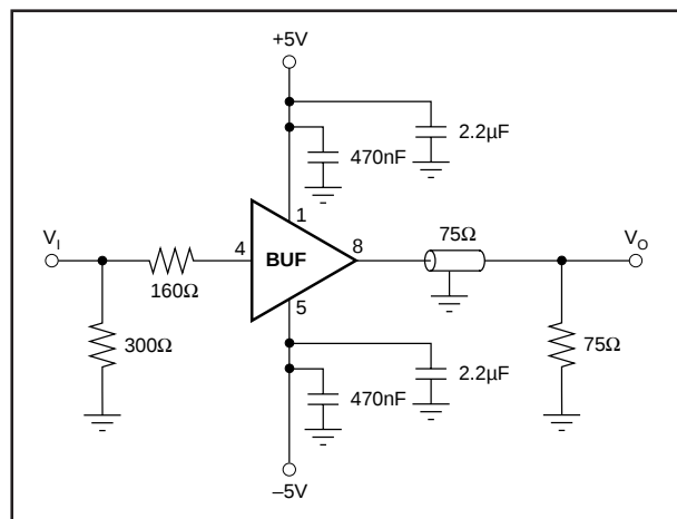
FIGURE 3. Impedance Converter.
