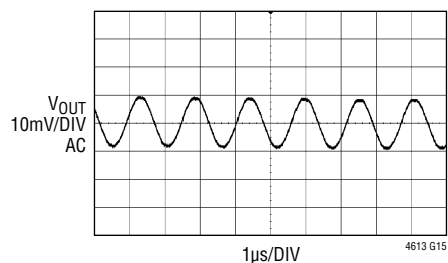
Output Ripple
