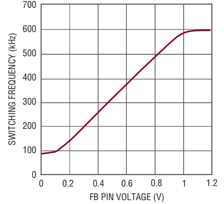
Frequency Foldback
