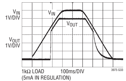
Start-Up/Dropout Performance
