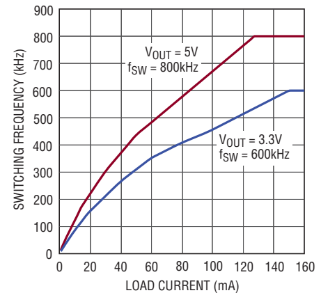
Burst Frequency
