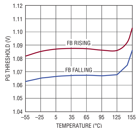
PG Thresholds
