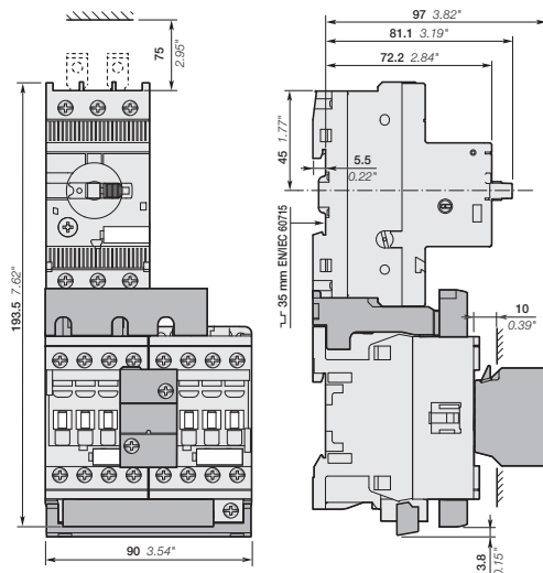
MS132-12 ... MS132-32 + BEA16-4 + AF09, AF12, AF16
