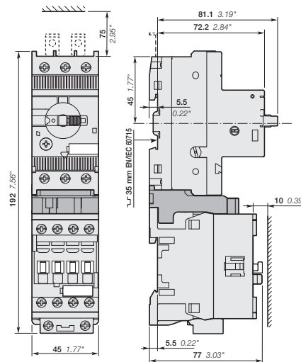
MS132-12 ... MS132-32 + BEA16-4 + AF09, AF12, AF16
