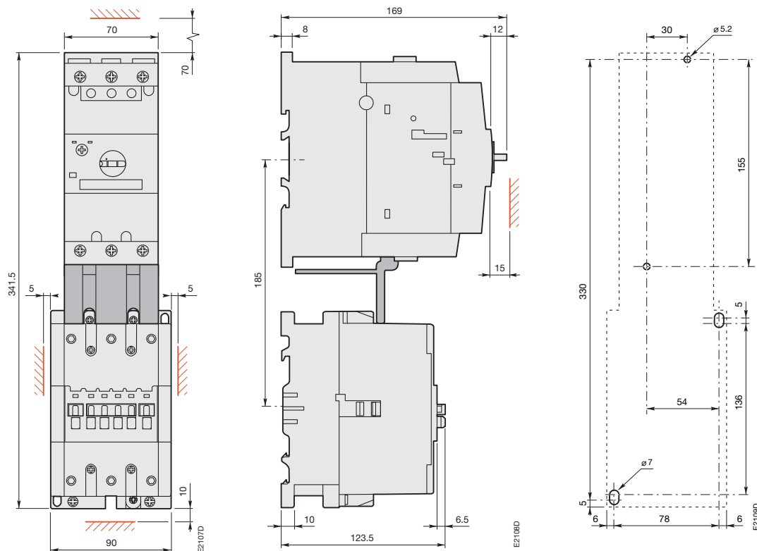
MS 49x + BEA 110/495 + A 95, A 110
