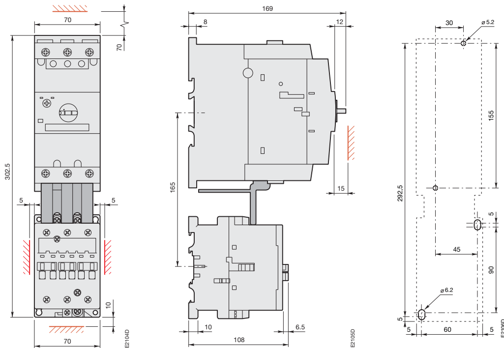
MS 49x + BEA 75/495 + A 50, A 63, A 75
