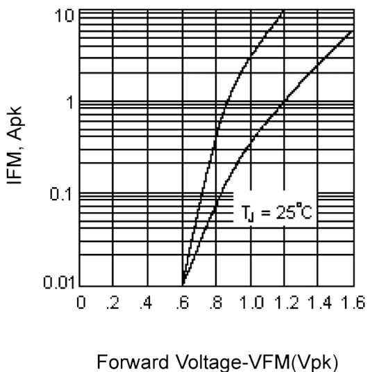
Figure 2 - Forward Characteristics
