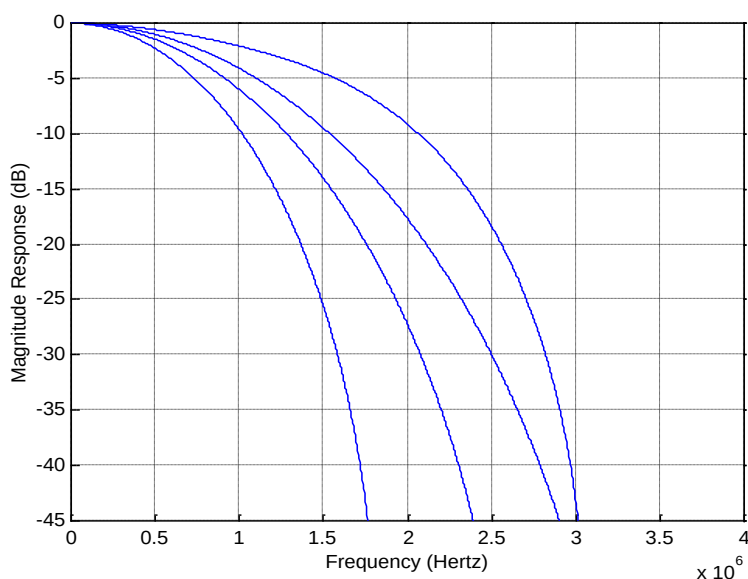
Fig6 The Characteristics of Chrominance Low Pass Filter
