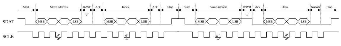
Fig13 Timing Chart of Serial Interface
