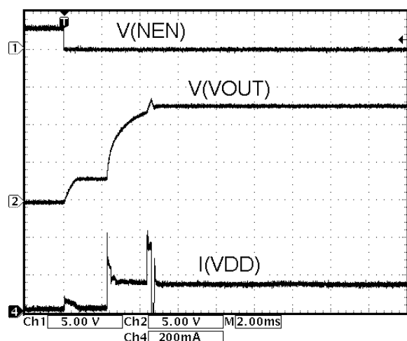
FIGURE 6. START-UP TO 12V @ SEL = 0 (V_{DD} = 3.6V, R_L = 360\Omega)
