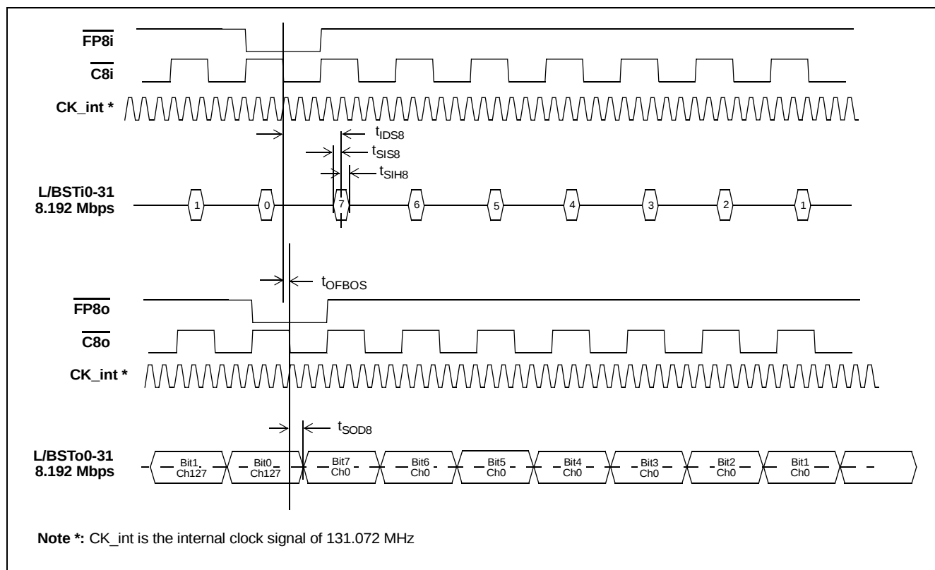
Figure 20 - ST-BUS Local/Backplane Data Timing Diagram (8 Mbps)
