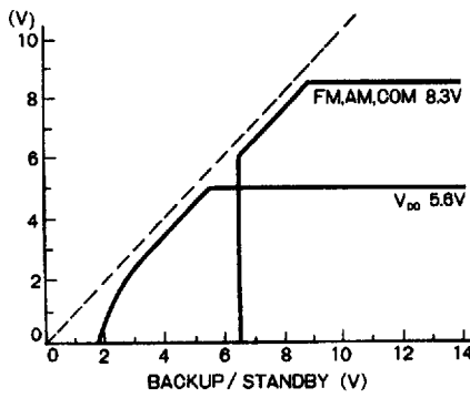
Figure 16 BA3906
