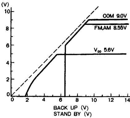
Figure 15 (BA3904A)
