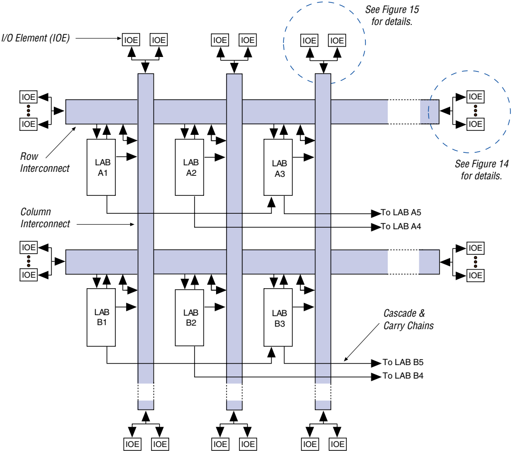
Figure 12. Interconnect Resources
