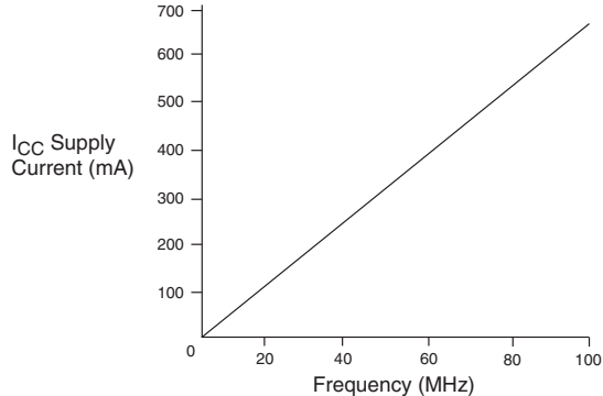
EPF10K50V
