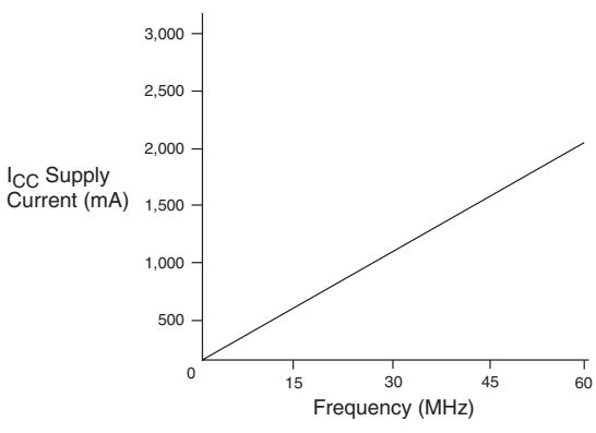
EPF10K50
