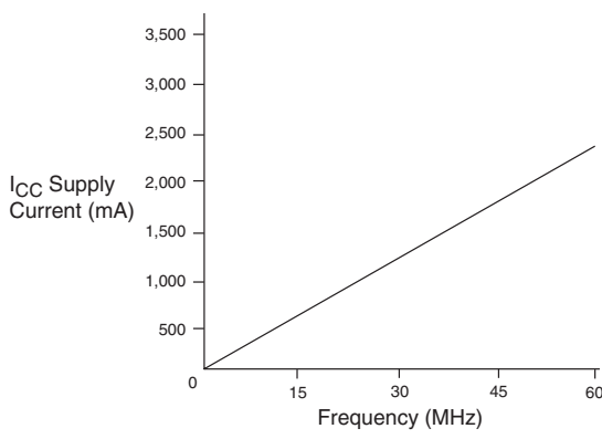
EPF10K70
